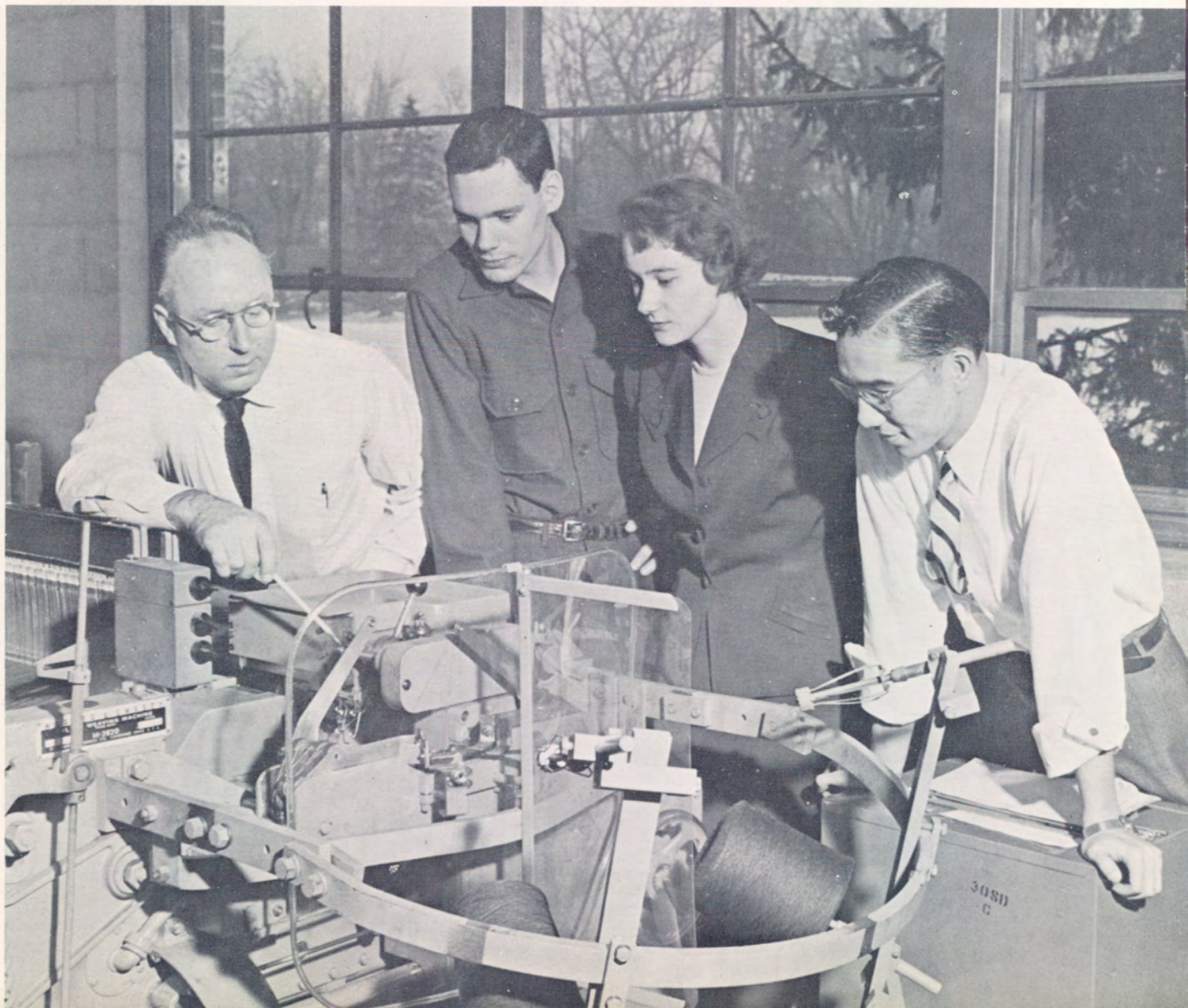
A laboratory lecture on the principles of the Warner and Swasey Sulzer Weaving Machine.
