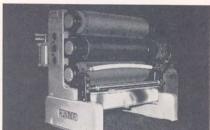
The Hunter 15-Ton 3-Roll Pad with 20" dia. cast iron body rolls and heavy-duty bearings for speeds up to 200 y.p.m. is adaptable to the most critical applications. A 10-Ton 2-Roll Pad, with 18" dia. rolls, delivers speeds to 150 y.p.m. Both feature individual pneumatic controls for either side of the Pad.
