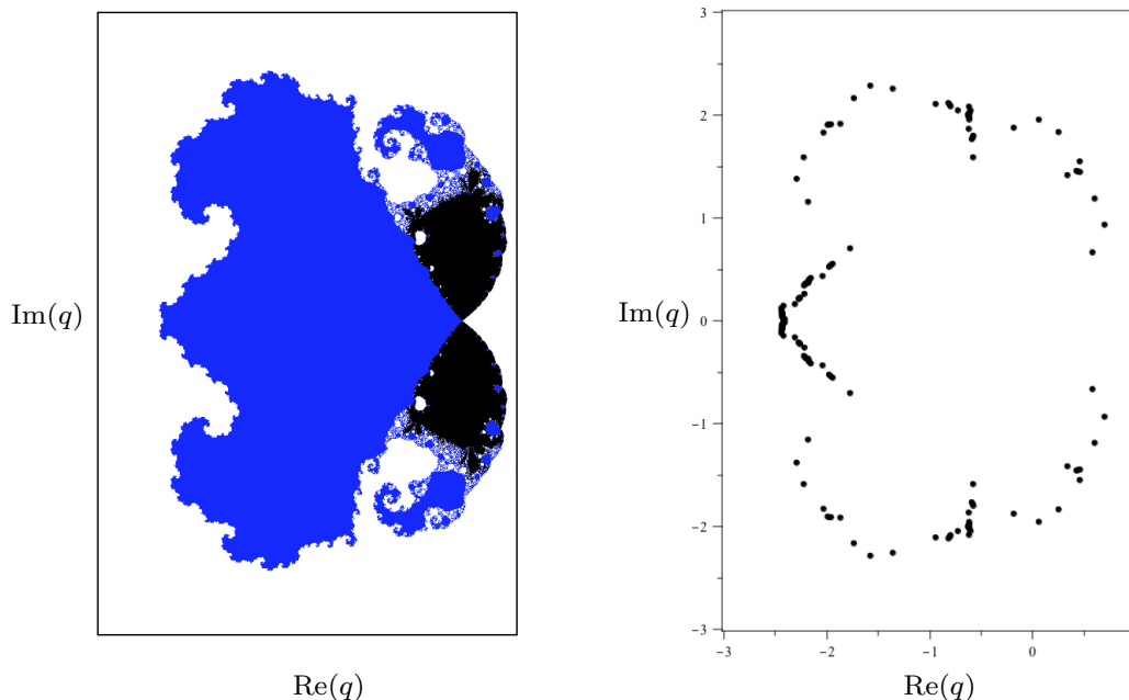
FIG. 9. Left: Region diagram for D_\infty in the complex q plane for \nu_0 = 1 . Right: Zeros of the reduced partition function Z_r(D_4, q, 1) (171 zeros). Both left and right figures depict -3 < \text{Re}(q) < 1 and -3 < \text{Im}(q) < 3 .
