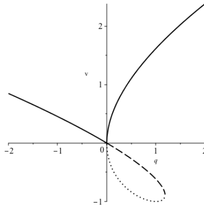
FIG. 2. Plot of the real fixed points of F_q(v) other than v = 0 and v = \infty . The v_{c,PM-FM}(q) fixed point exists for all q \in \mathbb{R} and is denoted by a solid line. The v_+(q) fixed point exists for 0 \leq q \leq \frac{32}{27} and is depicted by a dashed line. The v_-(q) fixed point for 0 \leq q \leq \frac{32}{27} is depicted by a dotted line.
