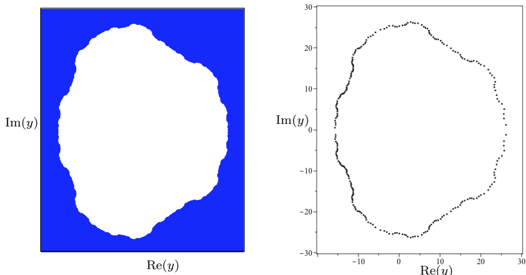
FIG. 14. Left: Region diagram for D_\infty in the complex y = v + 1 plane for q = 100 . The locus \mathcal{B}_v(100) is comprised of the boundary between the white and blue. (See text for further discussion.) Right: Zeros of the partition function Z(D_4, 100, y) (256 zeros). Both left and right figures depict -20 < \text{Re}(y) < 30 and -30 < \text{Im}(y) < 30 .
