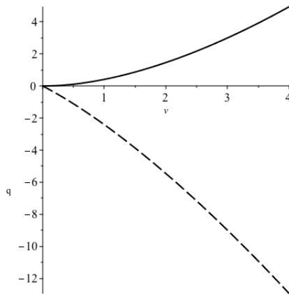
FIG. 13. Plot of the lower q_-(v_0) (dashed) and upper q_+(v_0) (solid) intersection points between \mathcal{B}_q(v_0) and the real q -axis for v_0 > 0 . See Theorem VIII.1.
