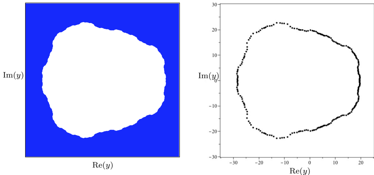
FIG. 15. Left: Region diagram for D_\infty in the complex y = v + 1 plane for q = -100 . The locus \mathcal{B}_v(-100) is comprised of the boundary between the white and blue. (See text for further discussion.) Right: Zeros of the partition function Z(D_4, -100, y) (256 zeros). Both left and right figures depict -35 < \text{Re}(y) < 25 and -30 < \text{Im}(y) < 30 .
