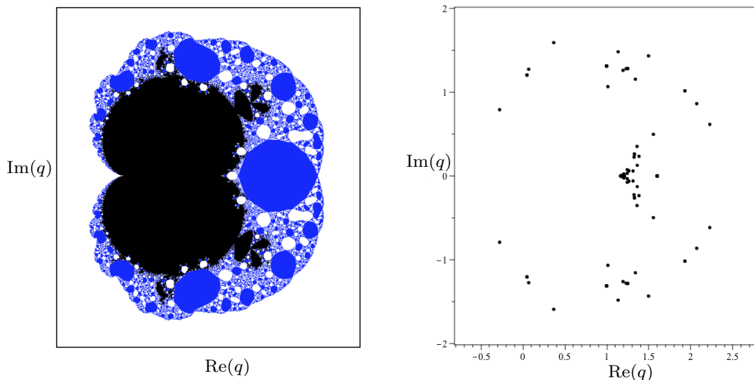
FIG. 5. Left: Region diagram for D_\infty in the complex q plane for \nu = -0.8 . Right: Zeros of the reduced partition function Z_r(D_4, q, -0.8) (171 zeros). Both left and right figures depict -0.8 < \text{Re}(q) < 2.8 and -2 < \text{Im}(q) < 2 .
