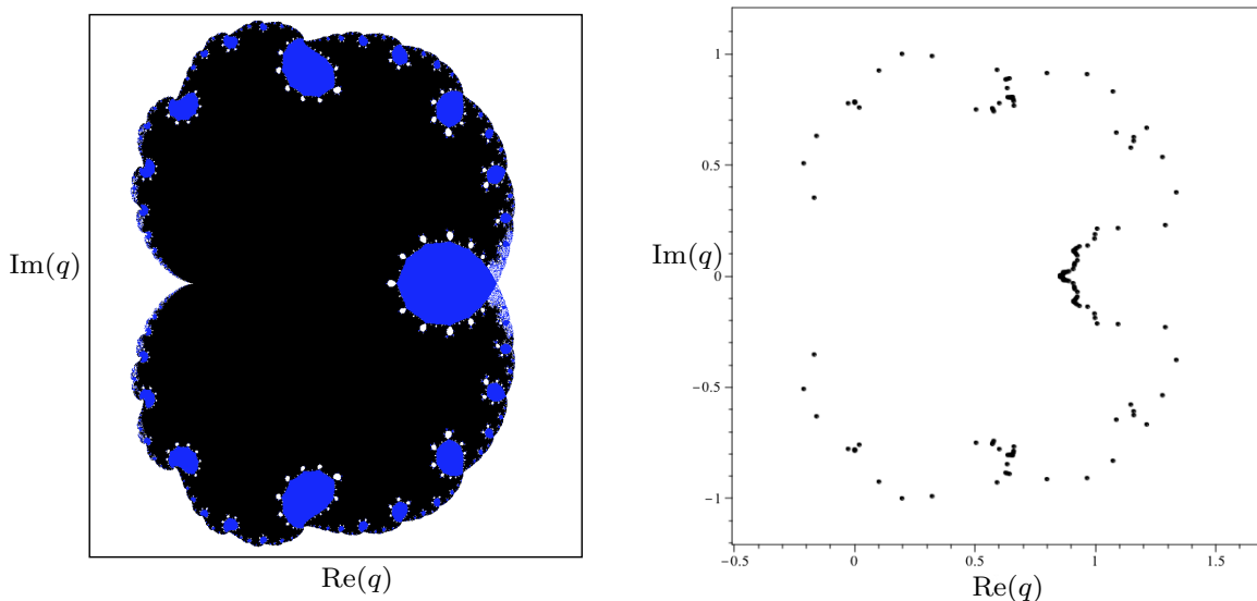
FIG. 6. Left: Region diagram for D_\infty in the complex q plane for \nu = -0.5 . Right: Zeros of the reduced partition function Z_r(D_4, q, -0.5) (171 zeros). Both left and right figures depict -0.5 < \text{Re}(q) < 1.7 and -1.2 < \text{Im}(q) < 1.2 .
