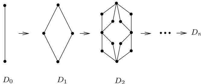
FIG. 1. Diamond hierarchical graphs D_m for m = 0, 1, 2 .
