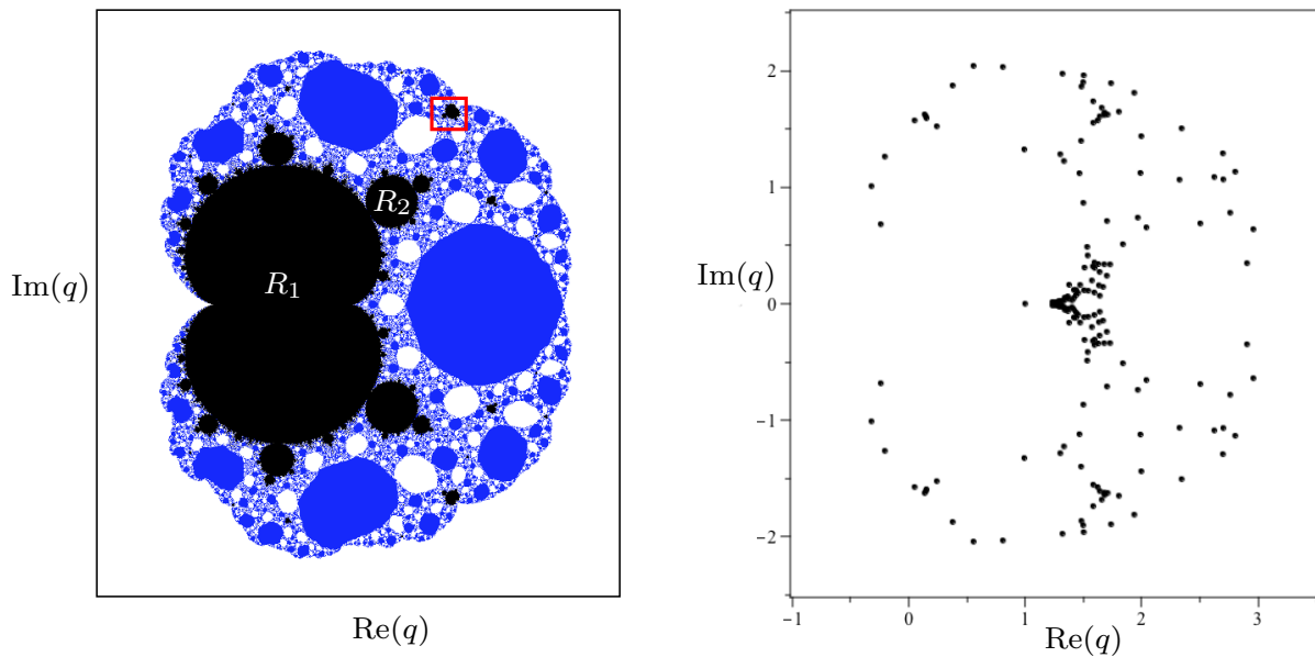
FIG. 3. Left: Region diagram for D_\infty in the complex q plane for \nu = -1 . The locus \mathcal{B}_q(-1) contains the boundaries between the white, blue, and black regions. It may also contain additional points in the black regions. (See Proposition V.7 and the paragraphs following it for further discussion.) The red box is referred to in the caption to Figure 4. Right: Zeros of the reduced chromatic polynomial P_r(D_4, q) = Z_r(D_4, q, -1) (171 zeros). Both left and right figures depict -1 < \text{Re}(q) < 3.5 and -2.5 < \text{Im}(q) < 2.5 .
