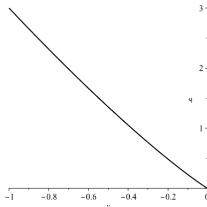
FIG. 8. Plot of the upper intersection point q_c(v_0) between \mathcal{B}_q(v_0) and the real q -axis for -1 \leq v_0 < 0 . See Theorem VII.1.
