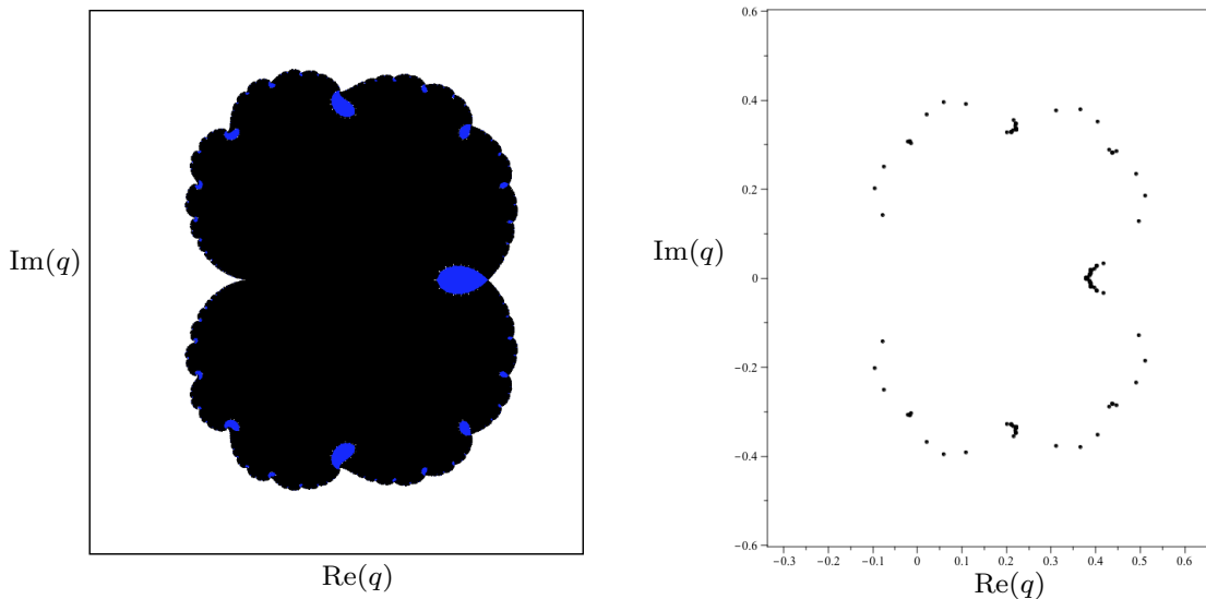
FIG. 7. Left: Region diagram for D_\infty in the complex q plane for v = -0.2 . Right: Zeros of the reduced partition function Z_r(D_4, q, -0.2) (171 zeros). Both left and right figures depict -1/3 < \text{Re}(q) < 2/3 and -0.6 < \text{Im}(q) < 0.6 .
