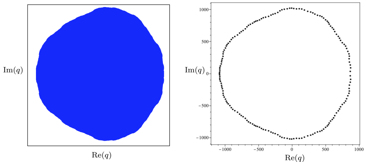
FIG. 12. Left: Region diagram for D_\infty in the complex q plane for v_0 = 99 . Right: Zeros of the reduced partition function Z_r(D_4, q, 99) (171 zeros). Both left and right figures depict -1200 < \text{Re}(q) < 1000 and -1100 < \text{Im}(q) < 1100 .
