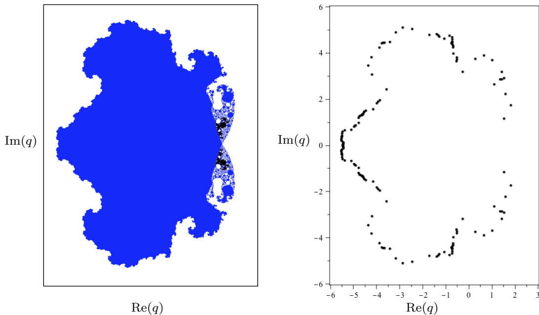
FIG. 10. Left: Region diagram for D_\infty in the complex q plane for v_0 = 2 . Right: Zeros of the reduced partition function Z_r(D_4, q, 2) (171 zeros). Both left and right figures depict -6 < \text{Re}(q) < 3 and -6 < \text{Im}(q) < 6 .
