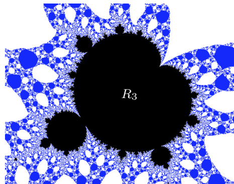
FIG. 4. Magnified view of area surrounded by the small red box from the region diagram on Figure 3. Here, \nu = -1 and 1.9 \leq \text{Re}(q) \leq 2.15 and 1.55 \leq \text{Im}(q) \leq 1.75 .
