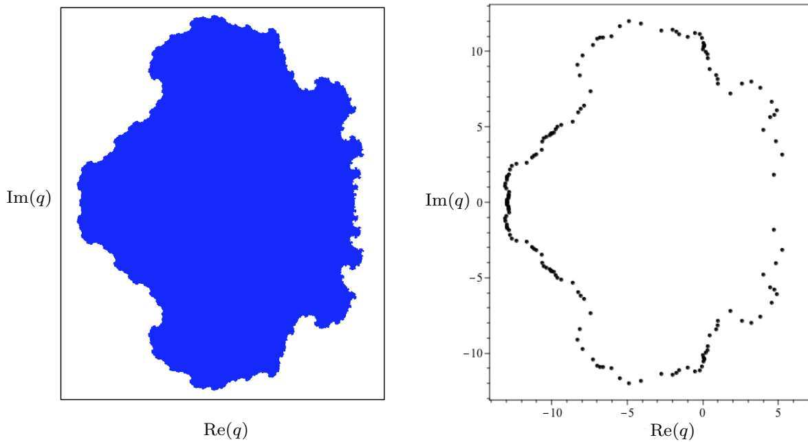
FIG. 11. Left: Region diagram for D_\infty in the complex q plane for v_0 = 4 . Right: Zeros of the reduced partition function Z_r(D_4, q, 4) (171 zeros). Both left and right figures depict -14 < \text{Re}(q) < 7 and -13 < \text{Im}(q) < 13 .
