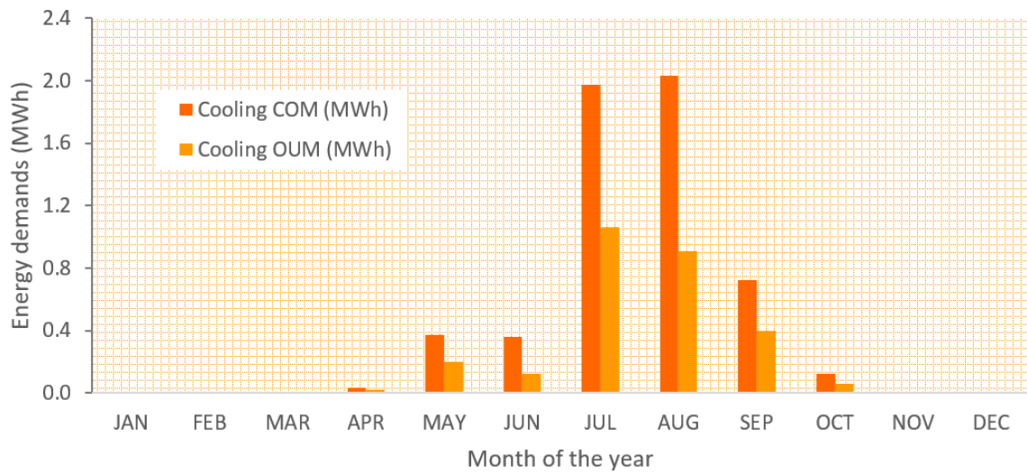
Figure 17. Monthly cooling energy demand of the surgical suite during COM and OUM.
