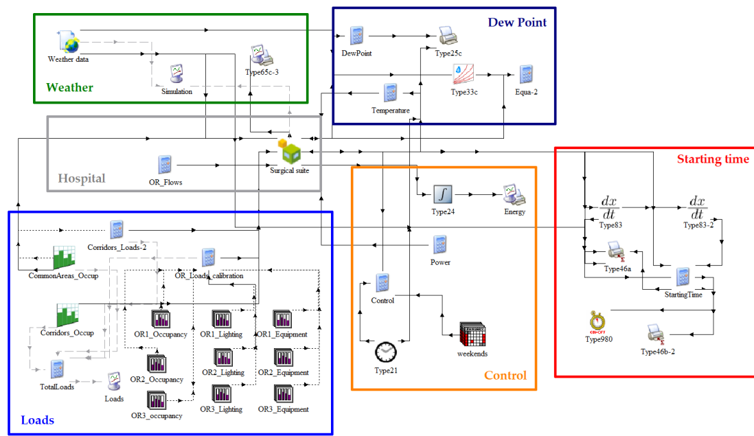
Figure 3. Simulation diagram implemented in TRNSYS.
