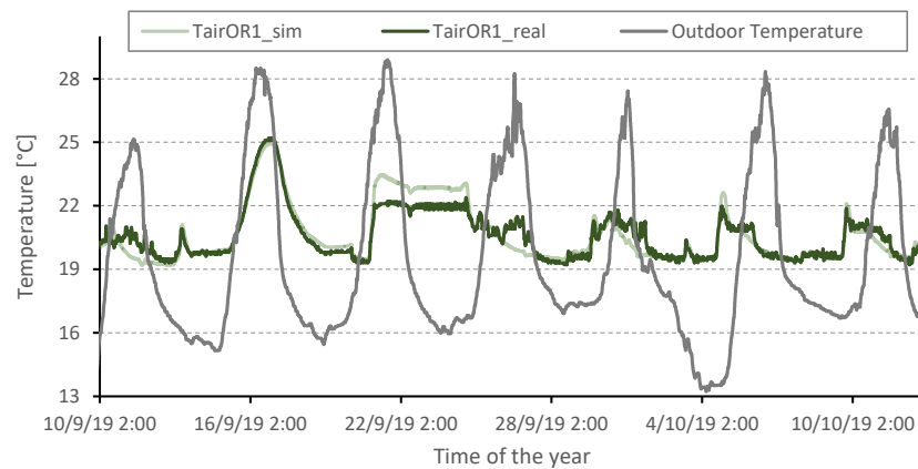
Figure 11. Comparison between measurements and simulation results for air temperature in OR1 during the second experimental campaign.
