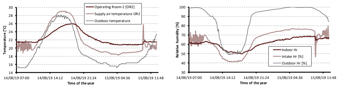
Figure 8. Temperature and RH in OR2 during the second experimental data campaign.
