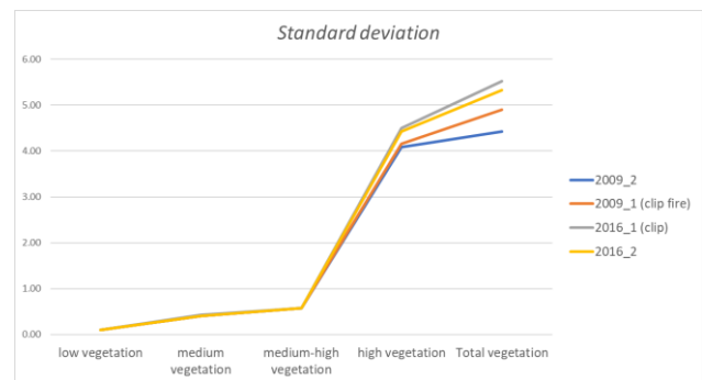
Figure 13. Standard deviation
