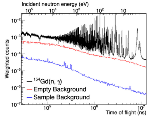
Fig. 2. Weighted spectrum measured with the ^{154}\text{Gd} sample compared to the background measured with an empty-sample holder and the one estimated from a measurement with a lead sample. The last spectrum was obtained by scaling the in-beam \gamma -ray background and the component due to the neutrons scattered by the sample, see text for details.
