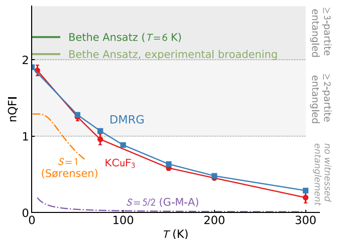
FIG. 5. Normalized quantum Fisher information [Eq. (7)] as a function of temperature. The y -axis units directly indicate the degree of multipartite entanglement present. When n\text{QFI} = f_Q/(12S^2) > m , where m > 0 is an integer, the system is in a state with \geq (m+1) -partite entanglement. We show n\text{QFI} densities calculated according to the formula in Eq. (4) from DMRG simulations and MAPS data. We also show theoretical n\text{QFI} calculated for a S=1 chain (“Sørensen”) [82] and for S=5/2 (“G-M-A”) [83]. Classical MC n\text{QFI} is zero at all temperatures.
