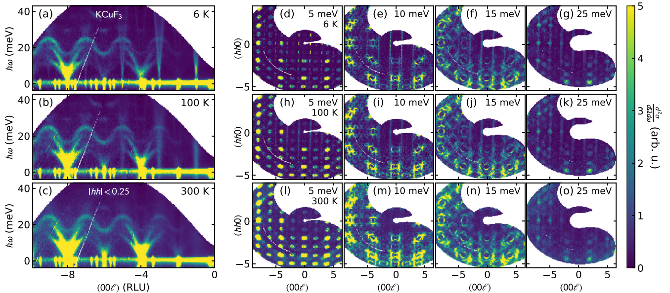
FIG. 8. Phonon spectrum for \text{KCuF}_3 . (a)–(c) show the phonon spectrum along (00\ell) , the direction of magnetic chains, at 6 K, 100 K, and 300 K, respectively. Magnetic scattering is visible as the strongly dispersive modes coming out of \ell = 1, 3, 5 , etc. (d)–(o) show constant energy slices ( \hbar\omega \pm 1 meV) at the three temperatures. The phonon spectrum is mostly below 30 meV and increases in intensity as temperature increases. Note that above 25 meV the phonons are mostly gone, leaving only magnetic intensity.
