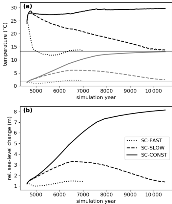
Figure 4. Temporal evolution of (a) global mean 2 m air temperature (black), ocean mean potential temperature (grey) and (b) relative sea-level change due to thermal expansion with respect to the starting point of each scenario. All plots show 30-year running means. The horizontal lines depict the value of the Marinoan control climate.
