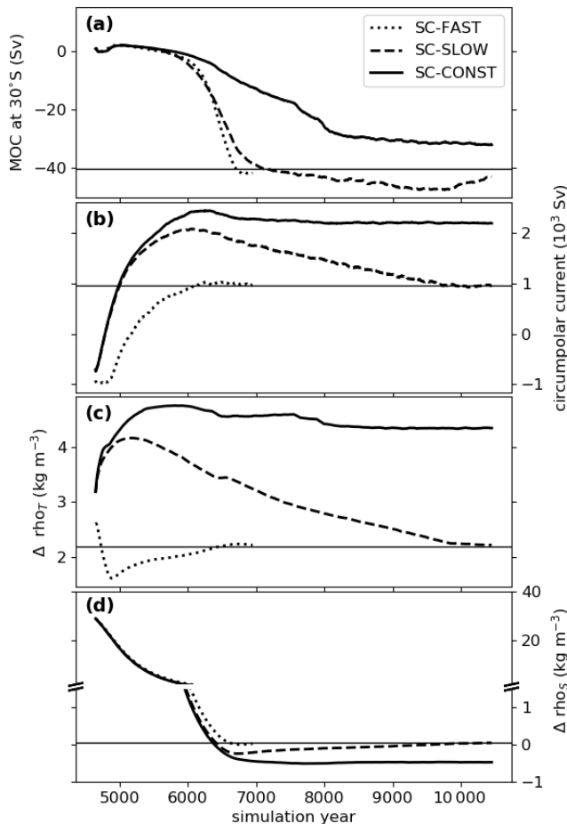
Figure 6. Temporal evolution of the large-scale ocean circulation. (a) Strength of the zonally averaged MOC at 30^{\circ} S and 1365 m depth. (b) Mass flux of the depth-integrated circumpolar current through a meridional section between the North Pole and the northernmost tip of the continents. Positive values refer to an eastward flow. (c) Global mean temperature contribution to the density difference from the ocean bottom to the surface. Higher values correspond to a stronger stratification. (d) Same as in (c), but for salinity; note the different scaling above and below the break in the y axis. The plots show 100-year running means. The black horizontal lines depict the mean value of the Marinoan control climate.
