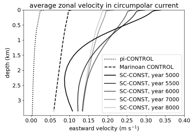
Figure 9. Vertical profiles of the zonally averaged eastward velocity component over the region of the circumpolar current. Shown are profiles from the pre-industrial control simulation (dotted), the Marinoan control simulation (dashed) and the scenario SC-CONST (solid) for the same times as the sections shown in Fig. 5. In the Marinoan setup, we define the region of the circumpolar current as the latitudes between 45 and 75° N, and in the present-day configuration the current is averaged over the latitudes between 75 and 45° S.
