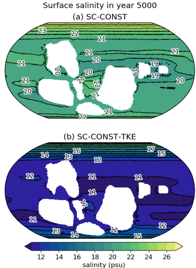
Figure 7. Surface salinity in year 5000 of (a) SC-CONST and (b) SC-CONST-TKE. The latter uses the parameters of the TKE vertical mixing scheme as they were suggested in Gaspar et al. (1990). The data in both plots represent a 30-year mean around the specified year.
