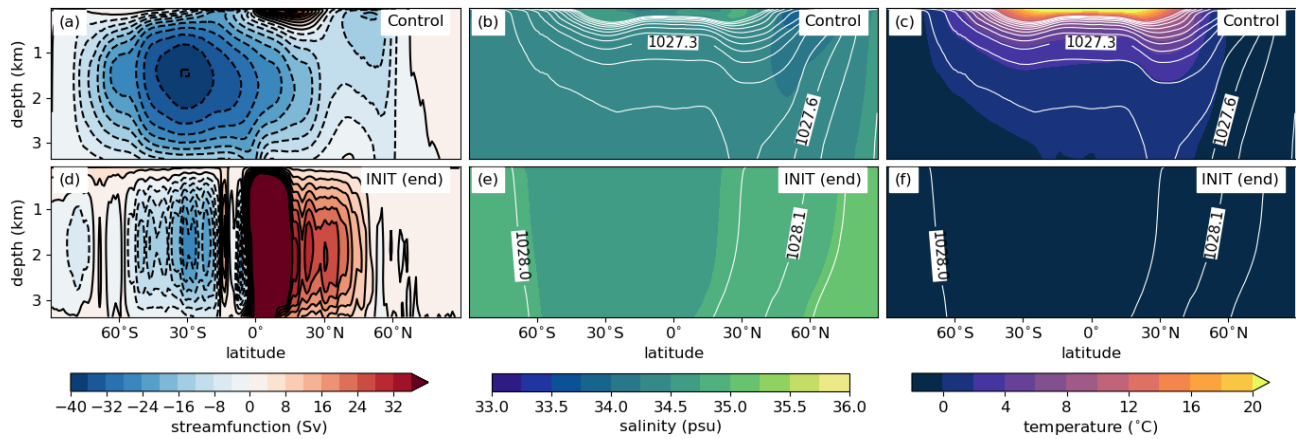
Figure 2. Zonal averages of ocean properties from the Marinoan control climate ( a, b, c ) and the end of the snowball initiation simulation INIT (averaged over the last 30 years, d, e, f ). The left column shows the meridional overturning circulation; negative values and blue shades refer to an anti-clockwise circulation. The middle and right columns show salinity and potential temperature, respectively. The white contours represent isolines of potential density in intervals of 0.1 \text{ kg m}^{-3} for densities above 1026.5 \text{ kg m}^{-3} .
