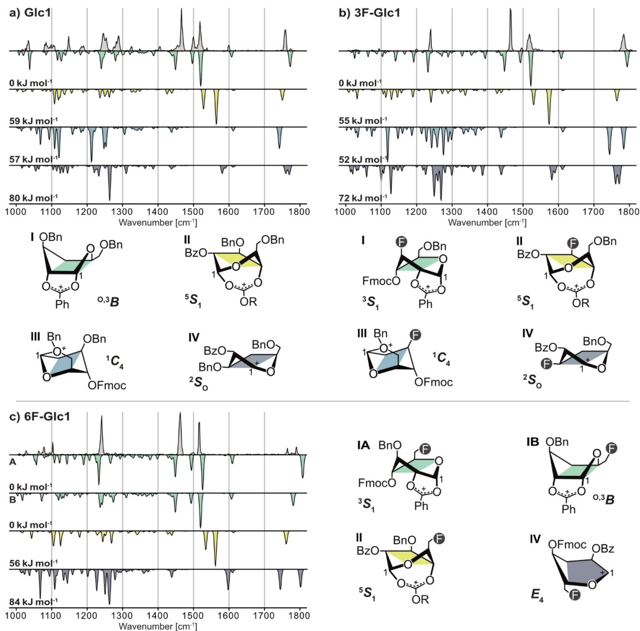
Figure 1. Infrared spectra of (a) Glc1, (b) 3F-Glc1, and (c) 6F-Glc1 glycosyl cations generated from \beta -thiotolyl (a) and \beta -thioethyl (b,c) precursors. Experimental IR spectra are shown as light gray traces. Computed spectra of lowest-energy dioxolenium structures, exhibiting neighboring group (green) and remote participation (yellow), oxonium (blue), and oxocarbenium structures (dark gray) are shown as inverted traces in respective colors. Relative free energies at 90 K are indicated. The lowest-energy structures are shown in a simplified representation below the spectra, with their ring pucker annotated. For clarity, some protecting groups have been omitted and R used as abbreviation for fluorenylmethyl. 3D-representation of the structures and xyz-coordinates can be found in the SI.
