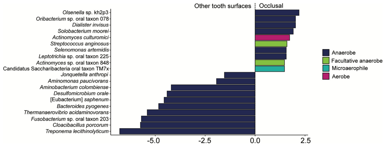
Figure 7. Differential abundance of taxa in occlusal samples compared to other tooth surfaces. Only the top 10 taxa are shown, and the bars are coloured by aerotolerance of the taxa.
