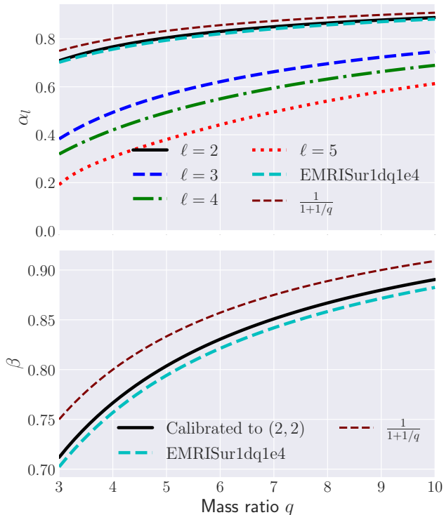
Figure 6. Scaling parameters \alpha_\ell(q) and \beta(q) as a function of mass ratio q . These parameters are obtained by minimizing the errors between ppBHPT and hybridized NR waveforms. In both panels, the dashed maroon line refers to a naive value of \alpha = \beta = 1/(1+1/q) set by including the mass of the smaller black hole as part of the background spacetime. We also show the scaling used in the previous model EMRISur1dq1e4 as a dashed cyan line in both panels.
