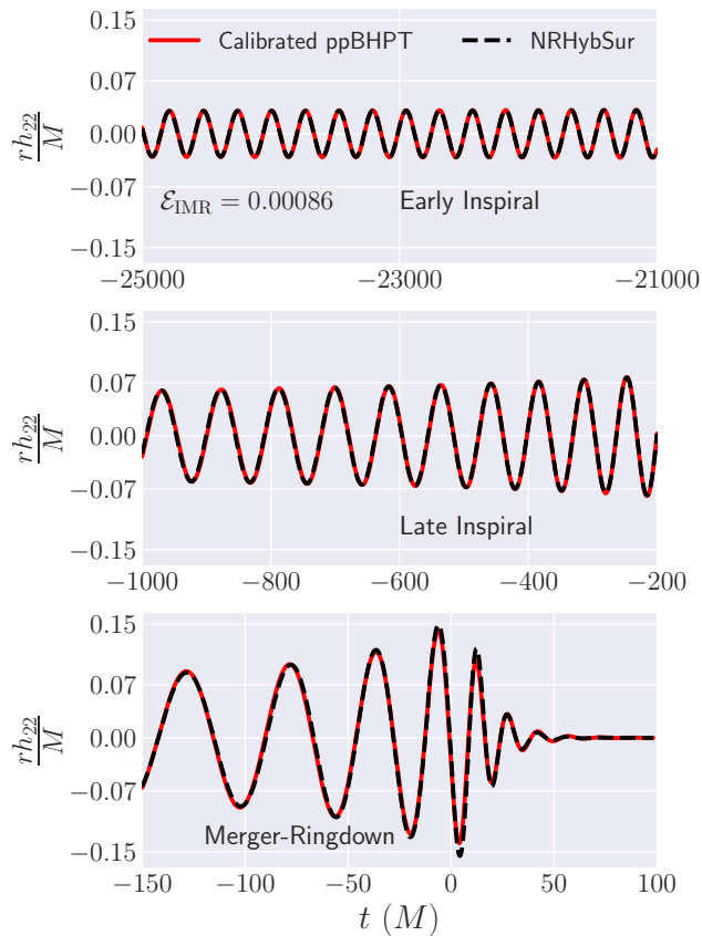
Figure 9. Effectiveness of the calibration obtained from a restricted time window [-5000, 115]M over the entire length of the waveform. Shown are the early inspiral (upper panel), late inspiral (middle panel), and merger-ringdown (lower panel) parts of the (2, 2) mode for q = 8 . The hybridized NR surrogate model NRHybSur3dq8 (referred as ‘ NRHybSur ’) and calibrated ppBHPT waveforms are shown in black dashed and solid red, respectively. \mathcal{E}_{\text{IMR}} is the L_2 norm error computed over the entire waveform.
