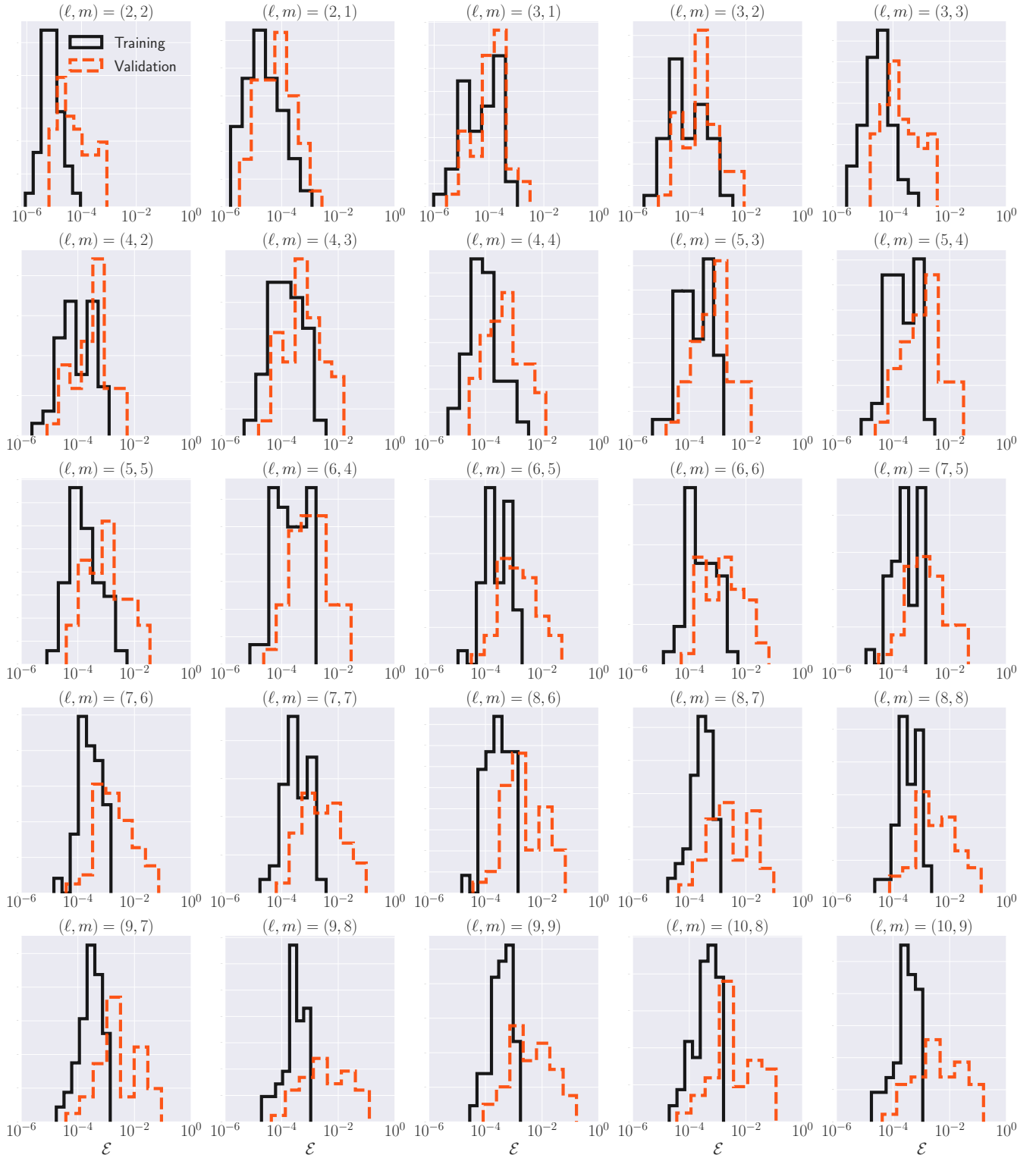
Figure 4. Time-domain errors \mathcal{E} , defined in Eq.4, for individual modes considered in BHPTNRSur1dq1e4. For comparison, we show both training (black solid lines) and validation (orange-red dashed lines) errors.
