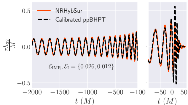
Figure 11. Comparison between the calibrated ppBHPT waveform and the hybridized NR surrogate model NRHybSur3dq8 (referred as ‘ NRHybSur ’) at q = 1.2 . We show the dominant (\ell, m) = (2, 2) mode. Errors for the full inspiral-merger-ringdown waveform and inspiral-only part are denoted by \mathcal{E}_{IMR} and \mathcal{E}_I , respectively.
