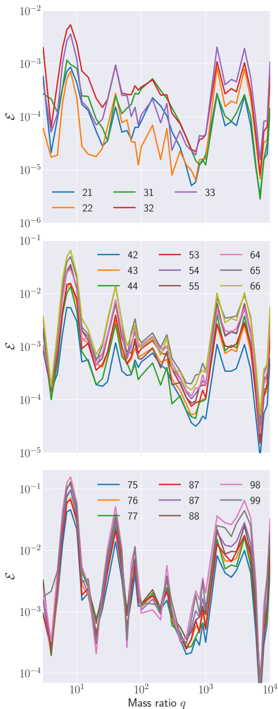
Figure 3. Validation errors, computed as \mathcal{E}[h^{\ell m}, h_s^{\ell m}] , for the individual modes in our surrogate model as a function of mass ratio q .
