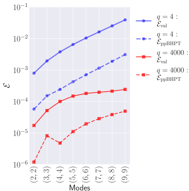
Figure 5. Validation errors (solid lines) and ppBHPT numerical errors (dashed lines) of select modes for two representative cases: q = 4 (blue circles) and q = 4000 (red squares).
