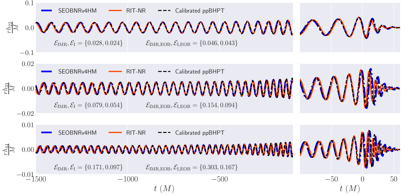
Figure 14. Waveform difference between the calibrated ppBHPT waveform (black dashed) and NR data (solid red) from the RIT group (simulation ID RIT:BBH:0792) for q = 32 . We show three different representative modes to demonstrate the efficacy of our model. Errors for the full inspiral-merger-ringdown waveform and only inspiral part is denoted by \mathcal{E}_{\text{IMR}} and \mathcal{E}_{\text{I}} respectively. For comparison, we also show SEOBNRv4HM waveform modes (solid blue).
