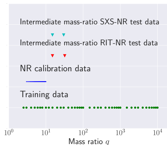
Figure 2. ppBHPT Waveform data points used in training BHPTNRSur1dq1e4 (green circles). We also show points used in calibrating the ppBHPT waveforms to NR (blue squares) and data points used in validating NR calibration against high mass ratio NR simulation (red and cyan triangles).
