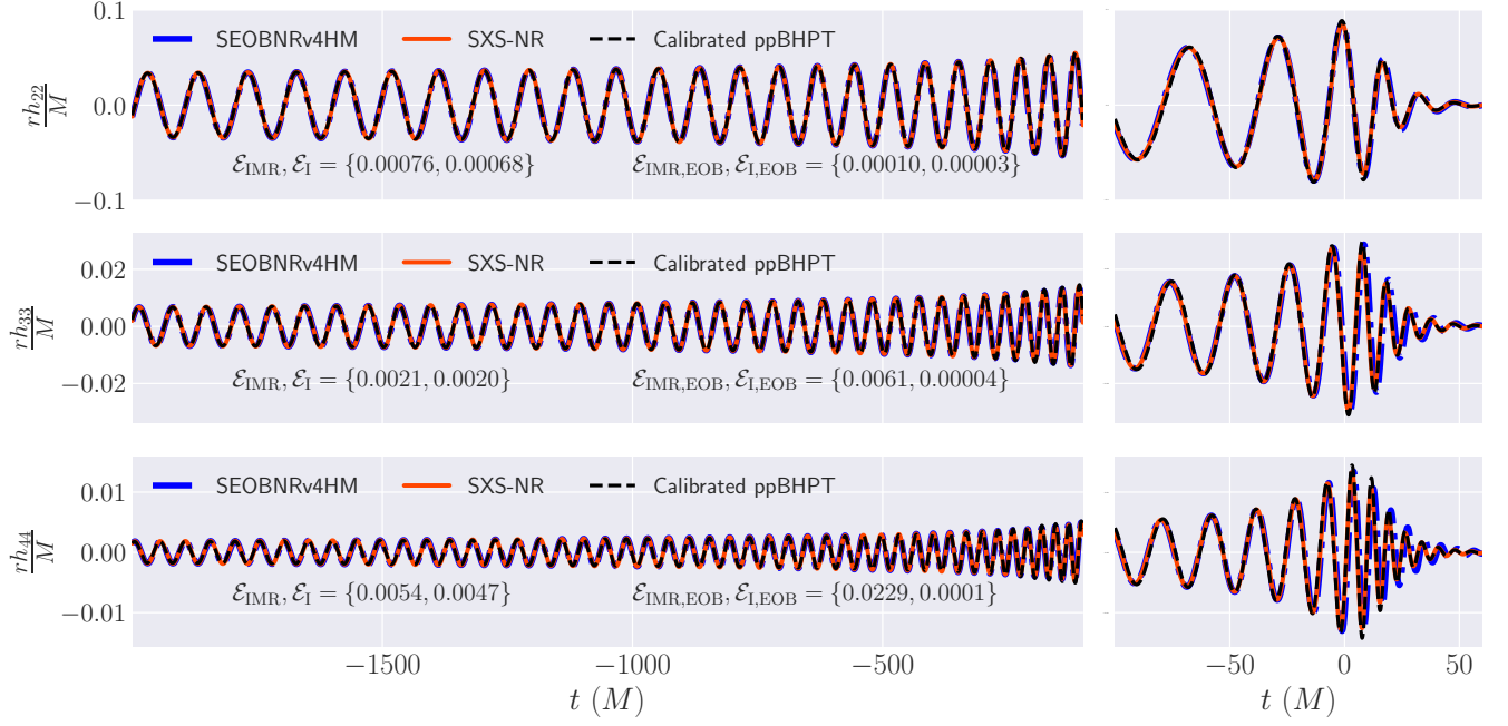
Figure 12. Waveform difference between the calibrated ppBHPT waveform (dashed black) and NR data (solid red) from the SXS collaboration (simulation ID SXS:BBH:2304) for q = 15 . We show three different representative modes to demonstrate the efficacy of our model. Errors for the full inspiral-merger-ringdown waveform and only inspiral part is denoted by \mathcal{E}_{\text{IMR}} and \mathcal{E}_{\text{I}} respectively. For comparison, we also show SEOBNRv4HM waveform modes (solid blue).
