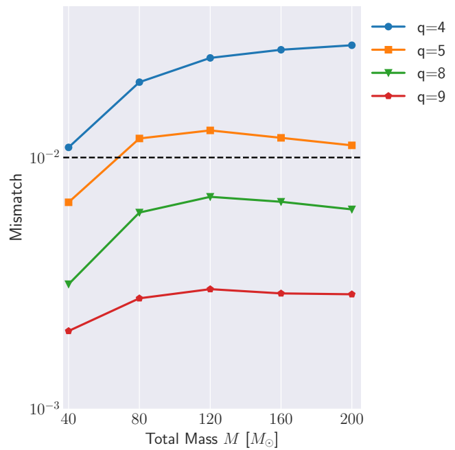
Figure 10. Frequency-domain mismatches between the rescaled-ppBHPT surrogate waveforms and NRHybSur3dq8 model for different mass ratios. The mismatches are shown as a function of the binary total mass M at inclination \iota = 0.0 and orbital phase \varphi = 0 , and are computed using the advanced LIGO design sensitivity noise curve. We set the minimum (maximum) frequency appearing in Eq. (17) to be 20Hz (990Hz). The dashed horizontal line demarcates a mismatch of 0.01, a commonly used threshold for sufficiently good model quality.
