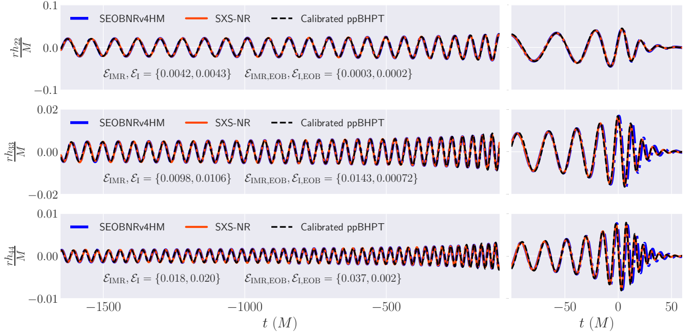
Figure 13. Waveform difference between the calibrated ppBHPT waveform (dashed black) and NR data (solid red) from the SXS collaboration for q = 30 [55]. We show three different representative modes to demonstrate the efficacy of our model. Errors for the full inspiral-merger-ringdown waveform and only inspiral part is denoted by \mathcal{E}_{\text{IMR}} and \mathcal{E}_{\text{I}} respectively. For comparison, we also show SEOBNRv4HM waveform modes (solid blue).
