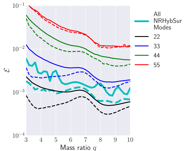
Figure 7. Time-domain error between the calibrated ppBHPT waveforms and the NR hybrid surrogate model as a function of mass ratio q . We show the errors computed over the full inspiral-merger-ringdown regimes (solid lines) and inspiral-only errors (dashed lines) restricting the waveform to t \leq -50M . We show errors for select modes ((2,2),(3,3),(4,4), and (5,5)) as well as for the case including all available NRHybSur3dq8 modes including \ell \neq m (referred as ‘All NRHybSur Modes’).
