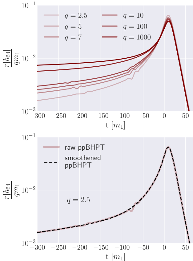
Figure 1. At mass ratios q \lesssim 10 the generalized Ori-Thorne transition trajectory causes small, nonphysical oscillations in some of the \ell \neq m modes. The raw ppBHPT waveform amplitudes are shown for one of the representative modes (\ell, m) = (5, 4) for increasing value of the mass ratio q (upper panel) and one example waveform after performing the smoothing procedure (lower panel) described in Sec. II C.
