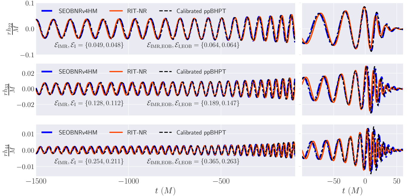
Figure 15. Waveform difference between the calibrated ppBHPT waveform (black dashed) and NR data (solid red) from the RIT group (simulation ID RIT:BBH:0373) for q = 15 . We show three different representative modes to demonstrate the efficacy of our model. Errors for the full inspiral-merger-ringdown waveform and only inspiral part is denoted by \mathcal{E}_{\text{IMR}} and \mathcal{E}_{\text{I}} respectively. For comparison, we also show SEOBNRv4HM waveform modes (solid blue).
