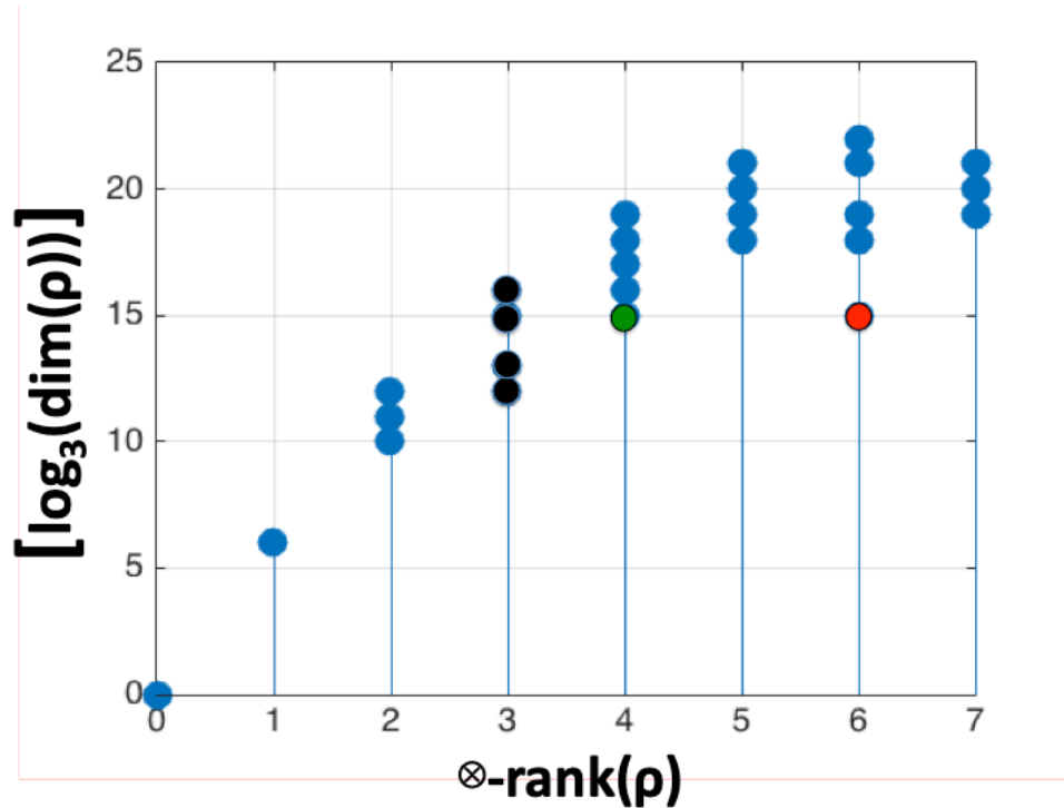
FIGURE 7. \log_q -scale of dimension vs. \otimes -rank for irreps \rho of GL_7(\mathbb{F}_q) , q = 3 .
