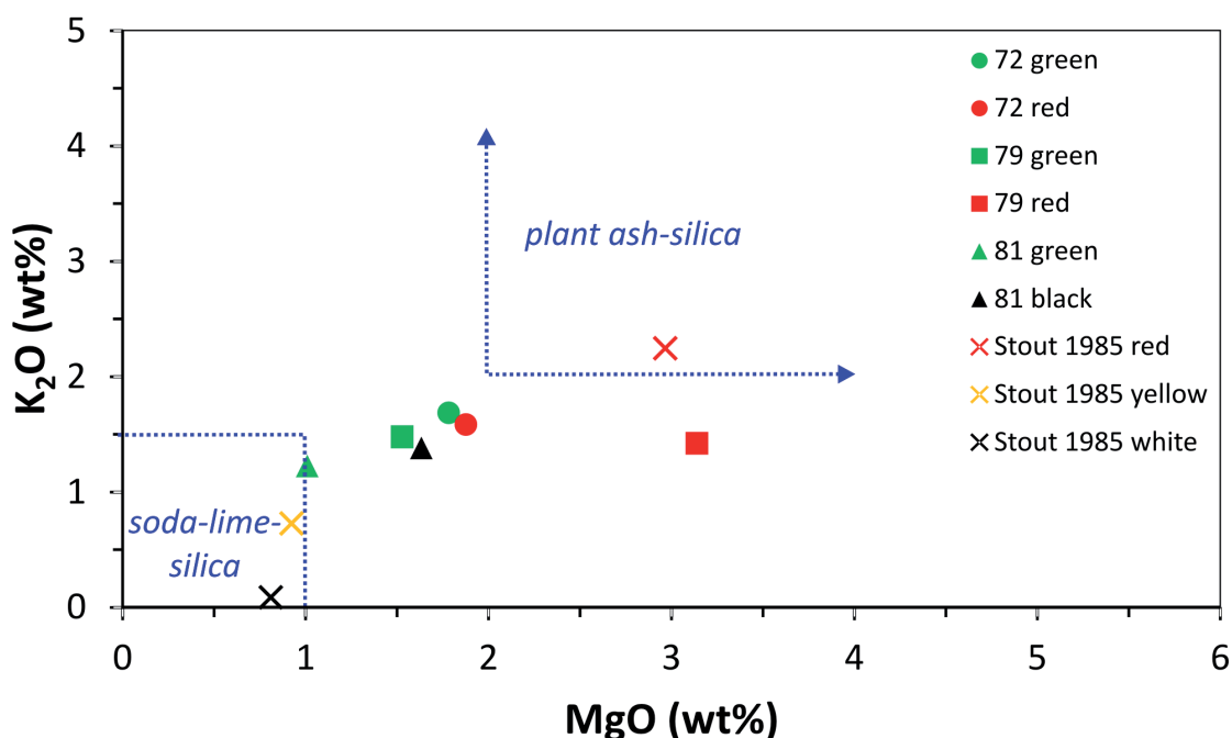
Fig. 3. The base glass composition of coloured (green, red and black) glasses of the face beads (calculated from the micro-XRF data) in the MgO vs. K 2 O binary diagram. Typical compositional ranges for soda-lime-silica and plant ash-silica glasses (after HENDERSON 2000 and FREESTONE 2005) as well as composition of white, yellow and red glasses of a face bead analysed by STOUT (1985) are indicated
