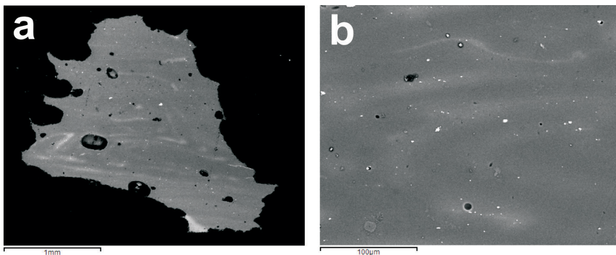
Fig. 2. Backscattered electron images of the green glass fragment detached from the rim of the face bead 72 showing tiny, bright, angular, antimony-based inclusions and lighter stripes in the vitreous matrix
