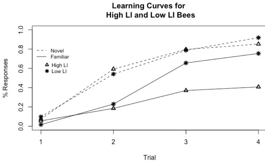
Fig. 1 Learning curves of LI phenotypes to a familiar and novel odor after the LI assay. Percent PER response over four trials are shown. Dashed lines represent the novel odor, while solid lines represent the familiar odor. Stars indicate low LI responses and triangles represent high LI responses
