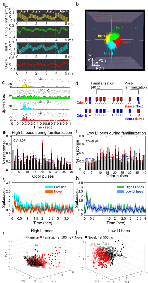
Fig. 3 Neural responses to familiar and novel odors. Individual units were separated from extracellularly-recorded waveforms (a) based on their distribution in the 3D principle component space (b). The responses of the 4 units in (a) are shown with their raster plots (40 stimulations) and peristimulus time histograms (PSTH) (c). Unit 2 did not produce an obvious response. Familiarity (or novelty) to odor A or B was introduced by stimulating the animal repeatedly 40 times with odor A or B (inter-pulse interval = 5 min; 4 sec duration) without any reward or punishment during the familiarization phase, and later tested during the post-familiarization phase (d). The averaged net responses (mean \pm SE) over the 40x repeated stimulation in the high LI bees (e) and low LI bees (f) show a large amount of trial-to-trial variation. The net response within a unit ( n=13 in high LI bees; n=12 in low LI bees) was normalized to the maximum of the 40 responses. The blue dotted lines represent 1st degree polynomial regression. CV: coefficient of variation. In Panel (g), the PSTHs (mean \pm SE) from all AL units regardless the type of bees show stronger response to the familiar odor (cyan) than to the novel odor (red) after familiarization. Similarly, the PSTHs from the high LI bees (green) show a higher transient response shortly after odor stimulation than the low LI bees (blue) (h). In both panels, odor onset was at time zero and stimulation lasted for 4 sec; the spike traces were binned at 10 msec resolution and the curves were Gaussian filtered with a moving window of 3 bins. Principle component analysis revealed that the ensemble dynamics to the familiar and novel odor stimulation in high LI bees were largely overlapped in the entire 4 sec of stimulation window, but showed apparent separation during the first 500 msec (filled red circles vs. filled black circles) (i). In low LI bees, the separation was less pronounced (j).
