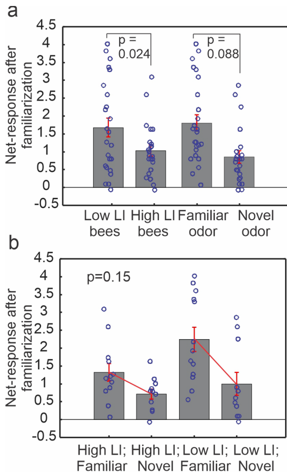
Fig. 4 Familiarization-induced responses to familiar and novel odors in high and low LI bees, analyzed with general linear mixed-effect modeling. The averaged post-netresponses (mean \pm SE; Cox-Box transformed) are plotted to compare the contributions of the fixed-effect terms to the model output. The p values indicate whether the coefficient of that term is significantly different from zero in the generalized linear model (see Methods). (a) Type of bees is a significant predictor ( p=0.024 , t test) with the low LI bees responding more strongly than the high LI bees; type of odors is a marginal predictor ( p=0.088 , t test) with the familiar odor eliciting stronger response than the novel odor. (b) The contribution of the interaction term (Odors X Bees) to the model is not significant ( p=0.15 , t test), indicating the response difference between familiar and novel odor was not dependent on the type of bees, evident from the nearly parallel lines across the bar graphs (mean \pm SE).
