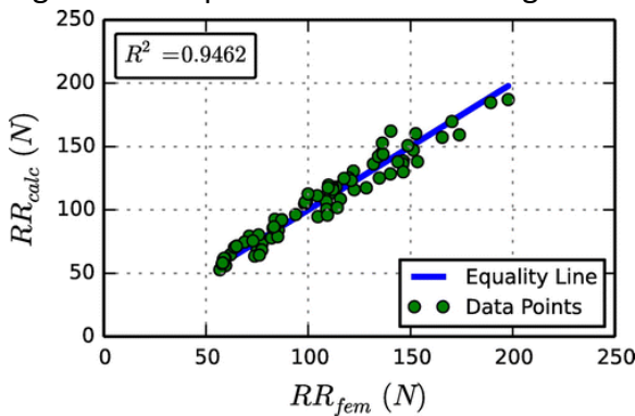
Figure 6. Comparison between rolling resistance from FE model and using Equation (5).
