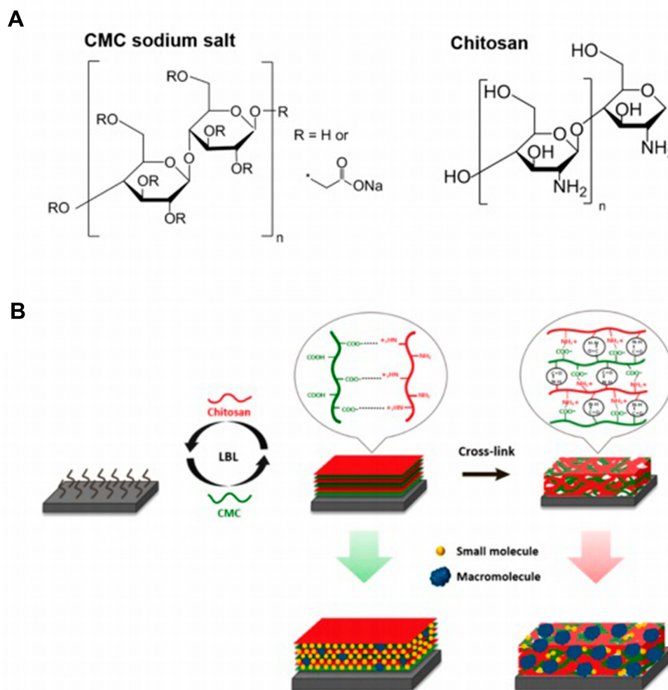
Figure 5 (A) Chemical structures of chitosan and carboxymethyl cellulose sodium salt. (B) Schematic illustration of the cross-linking-induced structural change of the LbL-assembled CMC/CHI multilayer film and its effect on the loading of drugs with different molecular weights.
