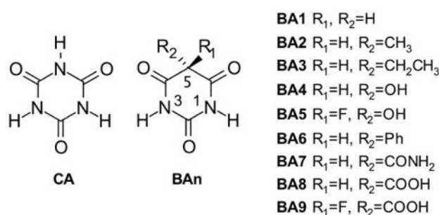
Scheme 1. Molecular structure of cyanuric acid (CA), barbituric acid (BA1) and some derivatives studied herein (BA n , with n = 1–9).
