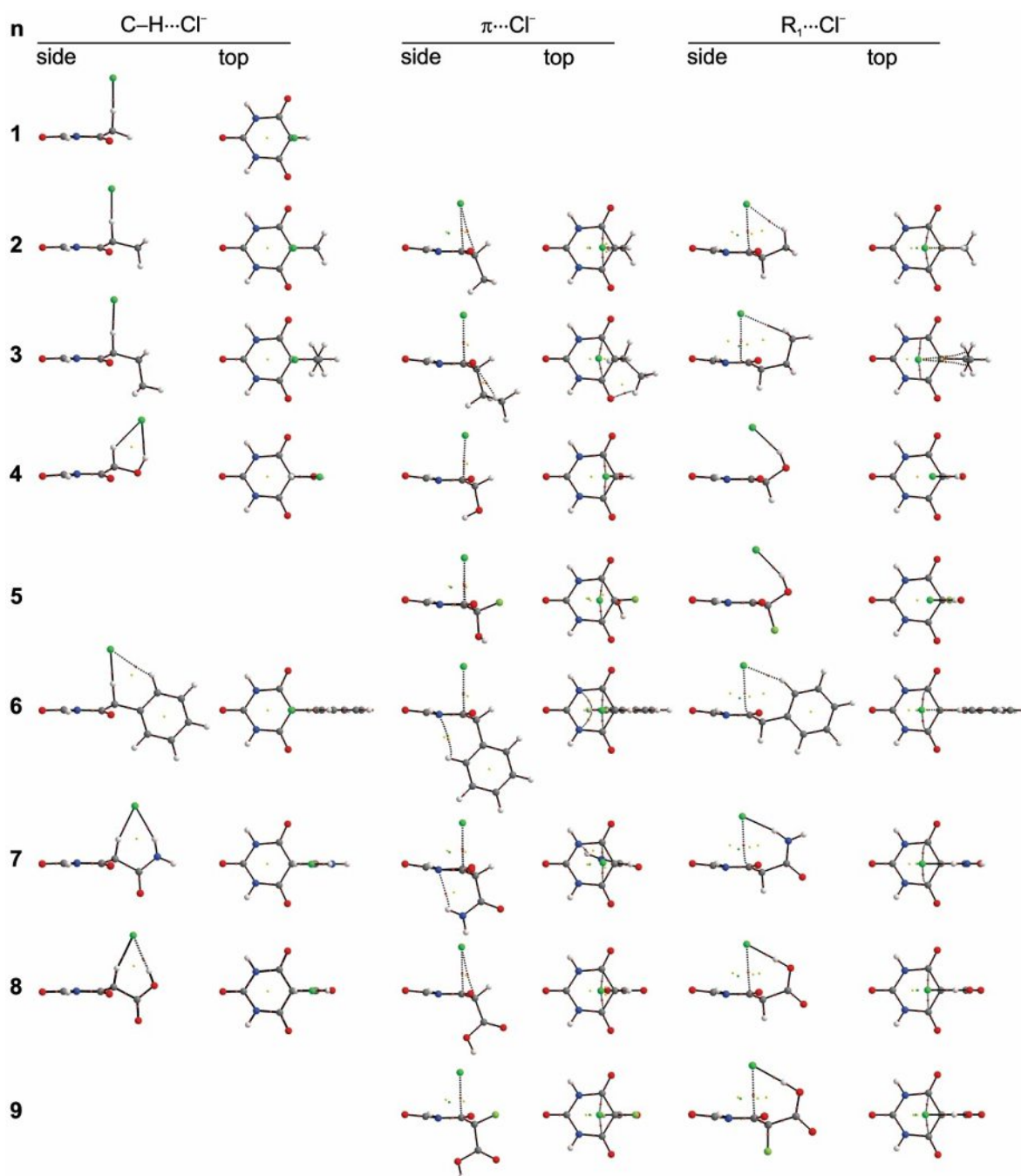
Figure 3. Top and side views of molecular graphs of BAn@Cl^- ( n = 1-9 ) complexes.
