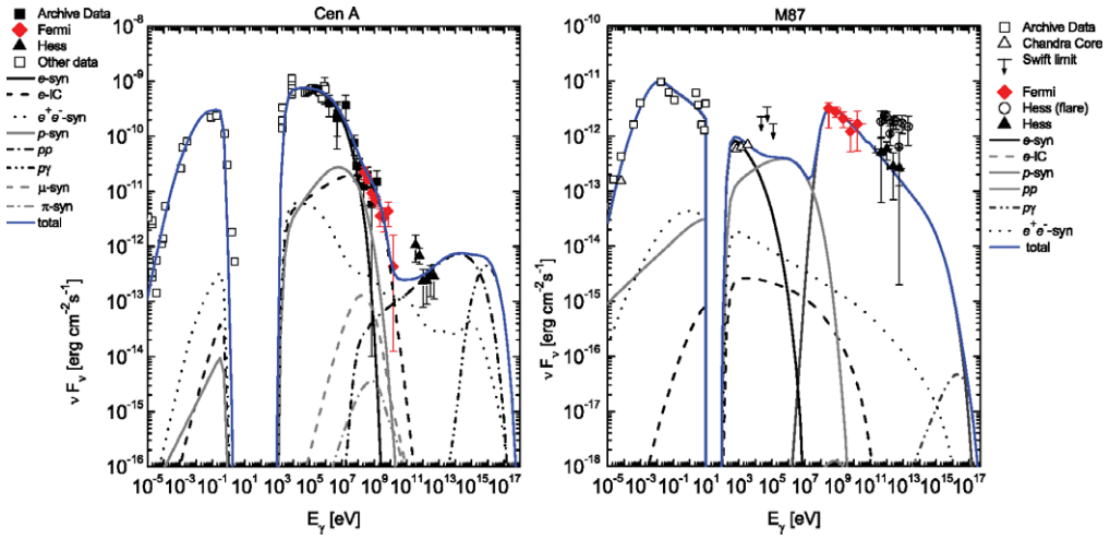
Figure 1. SEDs obtained for Cen A and M87.
