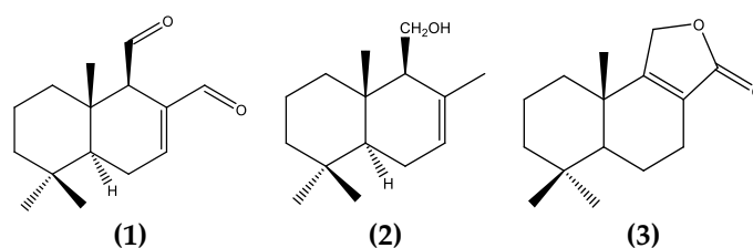
Figure 2. Chemical structures of the compounds isolated from Ethyl Acetate extract of leaves of Persicaria acuminata . (1) Polygodial; (2) Drimenol; (3) Confertifolin.
