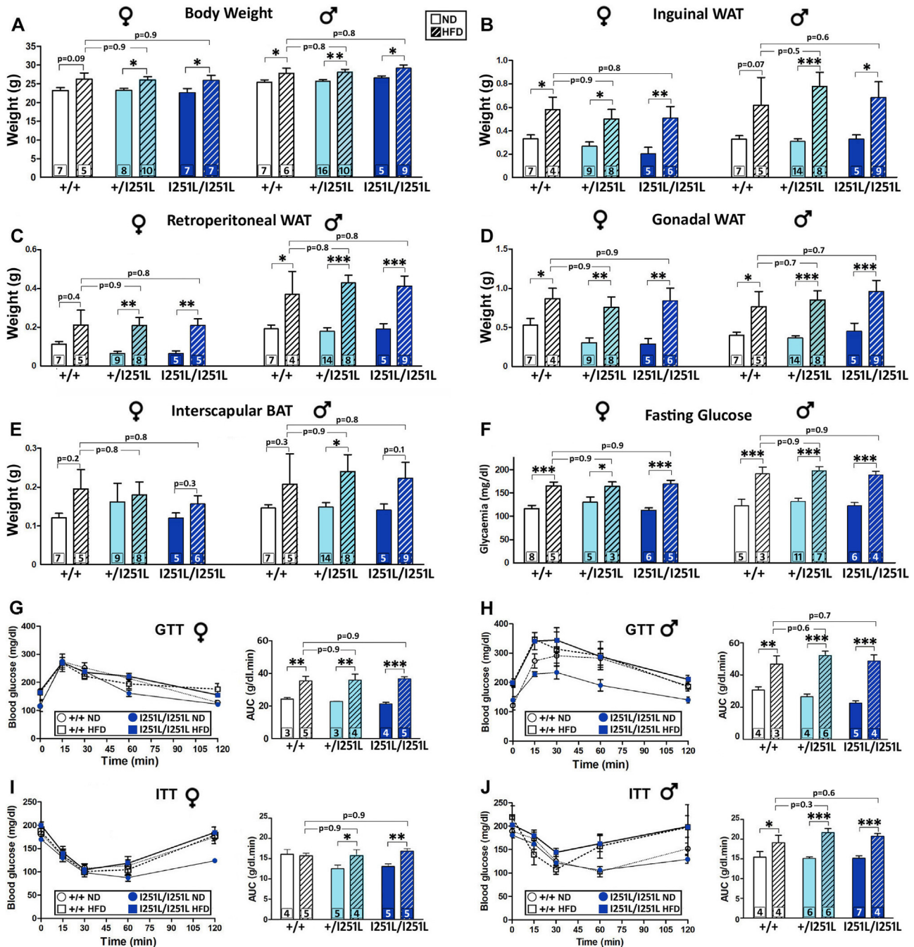
Figure 6: The I251L MC4R mutation does not protect against a high-fat diet. Metabolic phenotype of Mc4r^{+/I251L} and Mc4r^{I251L/I251L} females and males and their respective WT control littermates under the effect of a 3 month-high fat diet (HFD) compared to a normal diet (ND). (A) Body weight of 16-week-old mice ( n = 5-16 per group). (B–E) Determination of inguinal (B), retroperitoneal (C) and gonadal (D) white fat pads and interscapular brown fat pad (E) of 16-week-old mice. (F) Blood glucose concentration after 18 h of fasting in 15-week-old mice. (G–H) GTT using 1 g/kg D -glucose i.p. injection in 15-week-old females and males fasted 18 h. Bars represent the area under the curve. (I–J) ITT using 1 IU/kg human recombinant insulin (i.p.) in 15-week-old females and males fasted for 4 h. Bars represent the area under the curve. * P < 0.05 , ** P < 0.01 , *** P < 0.001 ; two-way ANOVA, Holm–Sidak. Values represent the mean \pm SEM of a number of mice per group indicated at the base of each bar.
