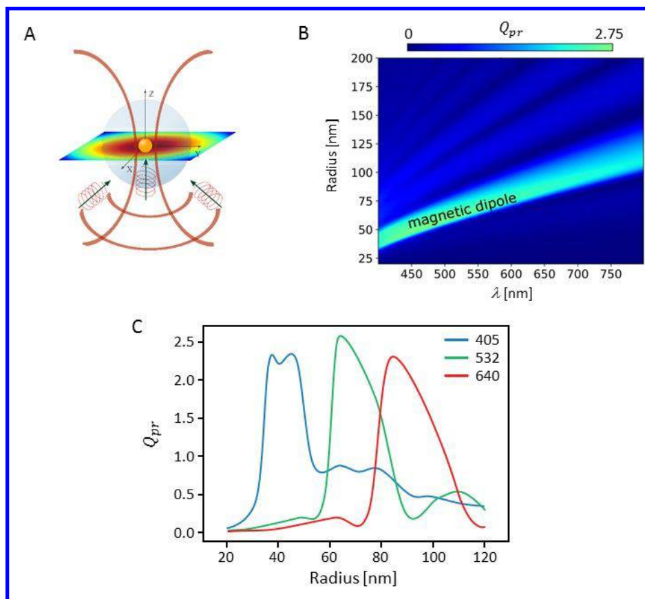
Figure 2: Radiation pressure efficiency for a Silicon nanosphere excited by a focused-dipolar laser beam when the particle is located at the focus center. (A) Laser beam scheme; (B) Dependency of radiation pressure efficiency Q_{pr} on the wavelength and the particle radius; (C) Q_{pr} vs. particle radius at three selected wavelengths used in the experiments: 405 nm, 532 nm, and 640 nm.
