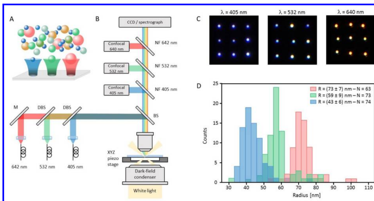
Figure 3. Size-selective optical printing of Si NPs. (A) Schematic of the size-selective optical printing process. (B) Sketch of the experimental set-up. (C) Example grids and (D) size distributions of NPs optically printed at 405 nm, 532 nm, and 640 nm.
