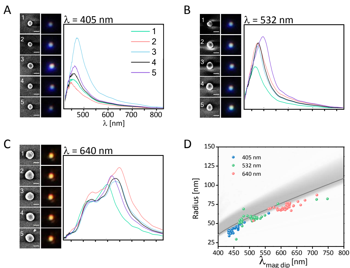
23 24 25 26 27 28 29 30 31 32 33 34 35 36 37 38 39 40 41 42 43 44 45 46 47 48 49 50 51 Figure 4. Size selectivity and optical properties of the optically printed Si NPs. (A-C) 52 Scattering spectra, dark field and FE-SEM images (scale bar = 100 nm) of selected single Si 53 nanoparticles printed at different wavelengths: (A) 405 nm, (B) 532 nm, (C) 640 nm; (D) 54 Radius vs. scattering maximum of the magnetic resonance for 115 Si NPs printed with the three 55 56 57 58 59 60
