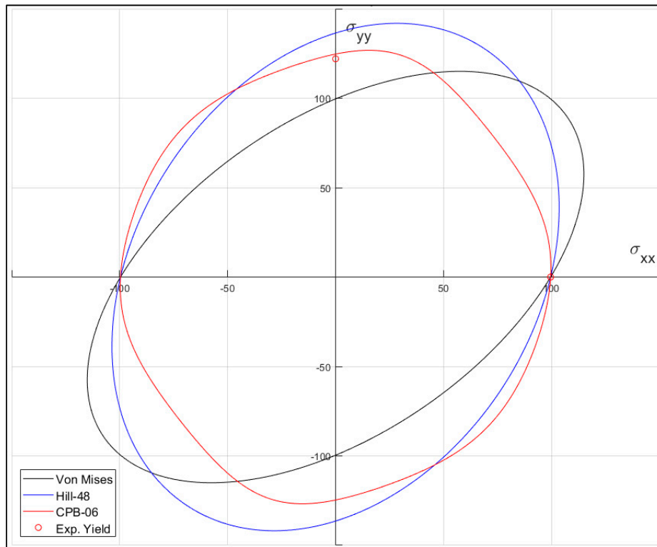
Figure 5. Plane stress yield envelope in the \sigma_{xx} | \sigma_{yy} plane at the yield strength for the von Mises, Hill-48 and CPB-06 criteria (the red circles denote the yield strengths for each sample direction).
