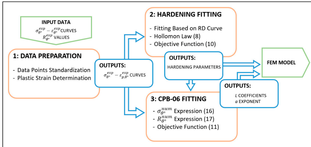
Figure 2. Flow diagram of the fitting procedure.
