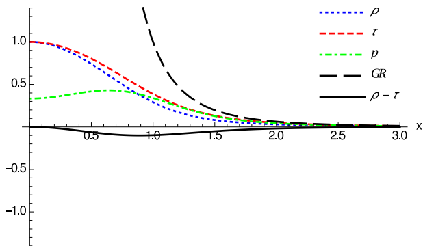
Figure 2. Graphical representation of the components \tilde{\rho} (blue dotted), \tilde{\tau} (red thin dashed) and \tilde{p} (green dashed-dotted) of the stress-energy tensor (24) as a function of x for regular horizonless solutions ( \delta_1 = \delta_c ) with N_q = N_c^\epsilon , which represents the transition case where the horizon disappears. At large distances all these components reduce to those of the Reissner-Nordström case (black thick dashed, upper curve in this figure), N_q/(N_c^\epsilon x^4) [see Eq. (31)]. The solid black line (lower curve in this figure) represents \tilde{\rho} - \tilde{\tau} < 0 , which means that the NEC is violated near the wormhole throat.
