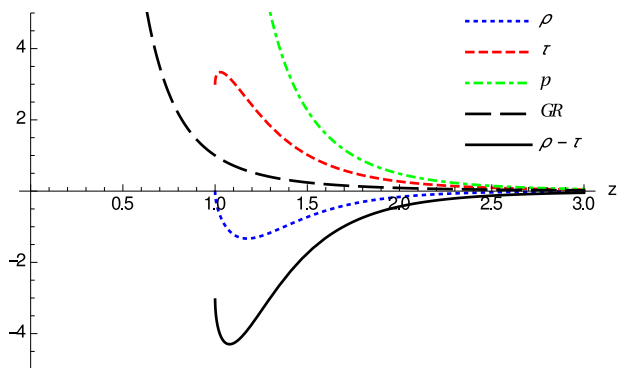
Figure 7. Same notation and curves as in Fig. 2, now for the f(R) gravity case with \alpha = 3/4 and parameters \delta_2 = 4\delta_1 and \delta_1 = 10 , for which no horizons are present. Note that the NEC is violated as \lim_{x \rightarrow 0}(\tilde{\rho} - \tilde{\tau}) < 0 (solid black) around the wormhole throat z = 1 . Note that though \tilde{\rho} < 0 near the throat, far away it becomes positive recovering the GR limit.
