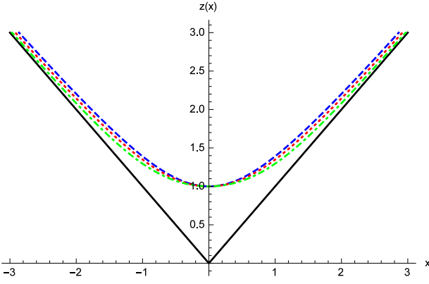
Figure 6. Behaviour of the radial function z(x) in the f(R) gravity case, obtained from Eq. (43), for the cases \alpha = 1/10, 1/3, 3/4 (dashed blue, dotted red and dotted-dashed green, respectively). At x \gg 1 the function z^2(x) \simeq x^2 and the GR behaviour is restored (straight solid black line). Observe the bouncing behaviour of all these curves at x = 0 .
