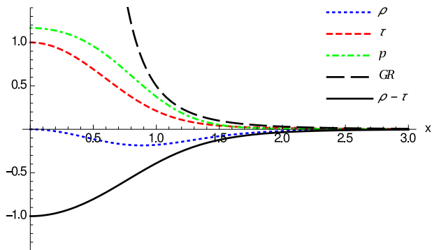
Figure 3. Same notation and curves as in Fig. 2, for \delta_1 = \delta_c now with N_q = N_c^\epsilon/2 (for l_\epsilon = l_P ). Here the NEC is violated because \tilde{\rho} - \tilde{\tau} < 0 (solid black). Note also that though \tilde{\rho} < 0 near the throat, far away it becomes positive ( \tilde{\rho} \approx q^2/r^4 ).
