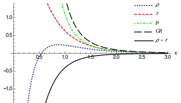
Figure 5. Same notation and curves as in Fig. 2, now with \delta_1 = \delta_c + 0.3 and N_q = N_c^\epsilon + 10 , corresponding to Reissner-Nordström-like configurations without horizons (naked). Note that the NEC is violated because \tilde{\rho} - \tilde{\tau} < 0 (solid black line) around the wormhole throat x = 0 . Here \tilde{\rho} and \tilde{\tau} diverge as 1/|x| when |x| \rightarrow 0 .
