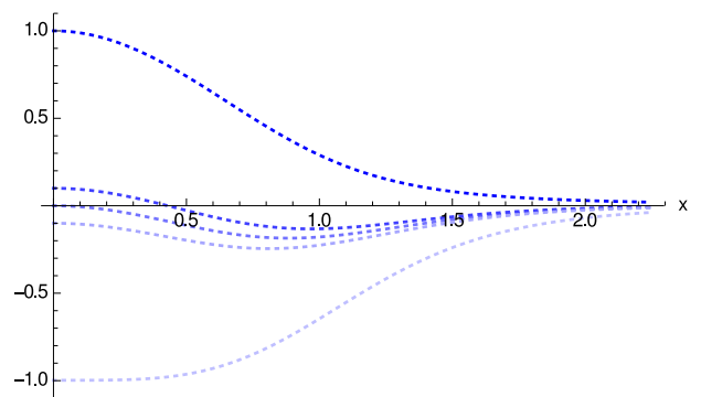
Figure 4. Representation of \tilde{\rho} for different values of N_q . The upper curve corresponds to N_q = N_c^\epsilon and the lower to N_q \rightarrow 0 . The middle curves represent, respectively, N_q > N_c^\epsilon/2 , N_q = N_c^\epsilon/2 and N_q < N_c^\epsilon/2 and illustrate how the energy density at the throat changes its sign as the number of charges decreases (in a continuum way).
