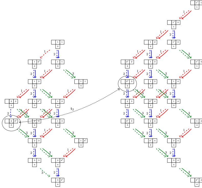
Figure 5.1: An example of the action of t_2 on a shifted tableau crystal \text{ShST}(\lambda/\mu, 4) , with \lambda = (3, 1) and \nu = (1) , which has two connected components.
