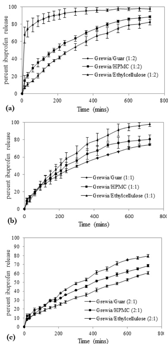
Figure 4 Release profiles of ibuprofen from the composite matrices containing 16% w/w of grewia and guar, HPMC, or ethyl cellulose in the ratio (a) 1:2, (b) 1:1 and (c) 2:1, in phosphate buffer solution at 37 \pm 1^\circ\text{C} (n=3, mean \pm s.d.)
