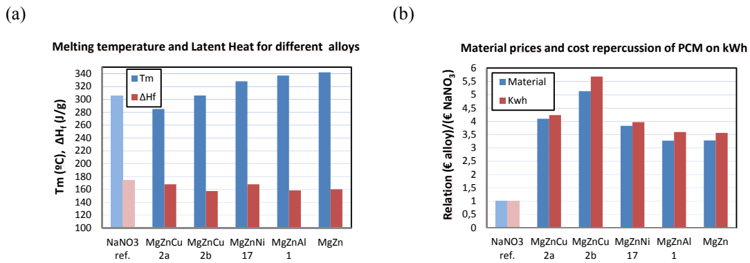
FIGURE 2. (a) Melting temperature and Latent Heat for the studied alloys (b) Material prices and cost repercussion of PCM on kWh. The material cost of NaNO_3 and its repercussion on the final price of kWh was taken as reference.
