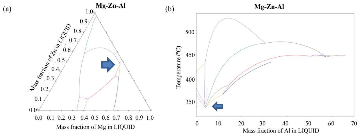
FIGURE 1. (a) liquidus surface projection into the composition axis of Zn and Mg. (b) liquid monovariant line of the Al composition plane. The arrows correspond to the minimum liquidus temperature for 3.97Al-49Mg-47Zn (wt%)
