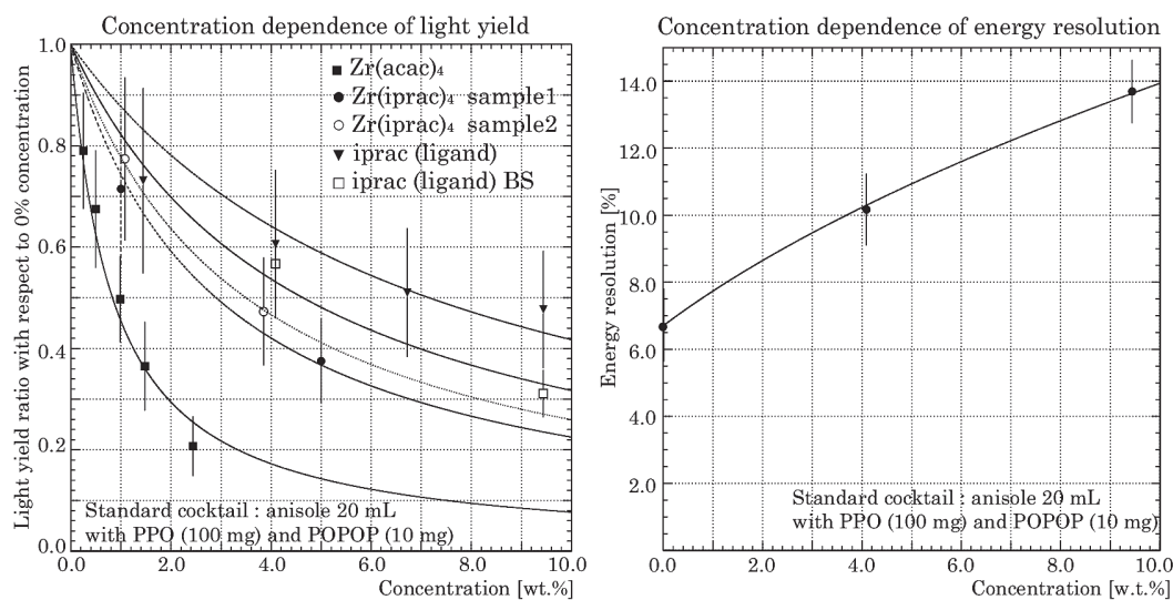
Figure 8. Light yield fraction as a function of the concentration of Zr(iprac)_4 and isopropyl acetoacetate (left panel). Measured energy resolution as a function of the concentration of Zr(iprac)_4 and isopropyl acetoacetate (right panel).
