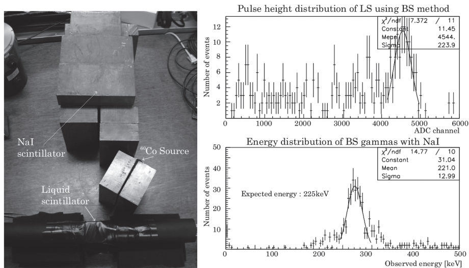
Figure 6. Setup for measurement of the single peak for the liquid scintillator using the backscattering method.
