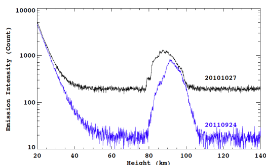
Figure: Comparison of LIDAR data (vertical direction) between October 27, 2010 (black) and September 24, 2011 (blue). Integration time is 5-sec.
