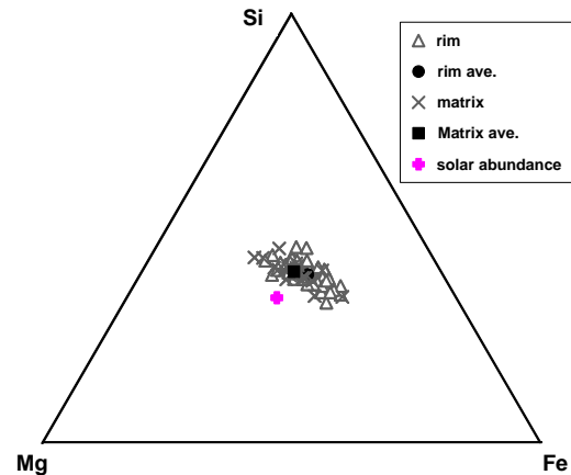
Fig. 2. Ternary Si-Mg-Fe wt% diagram for chemical composition of rim and matrix in ALH 77307 (CO3.0).
