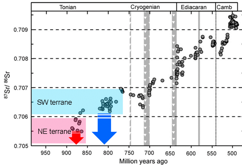
Figure 2. Based on Halverson et al., 2010, the depositional age of carbonate rocks can be estimated from initial Sr isotope ratio. Carbonate rocks from the NE terrane were most likely to have deposited around 770-850 Ma and those from SW terrane were deposited around 890-850 Ma.
