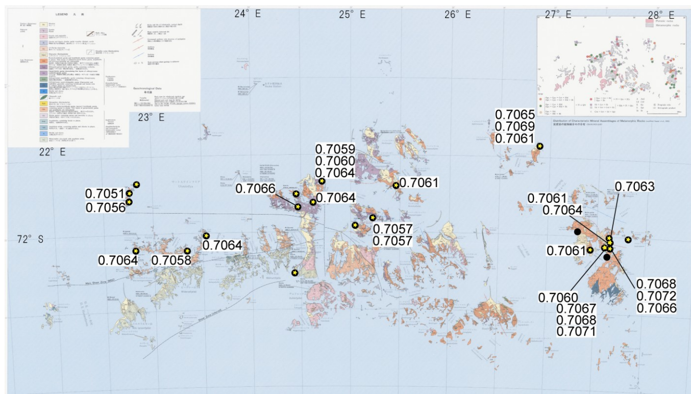
Figure1 Geological map of Sør Rondane Mountains showing the sampling site of meta-carbonate rocks and ^{87}\text{Sr}/^{86}\text{Sr} ratio
