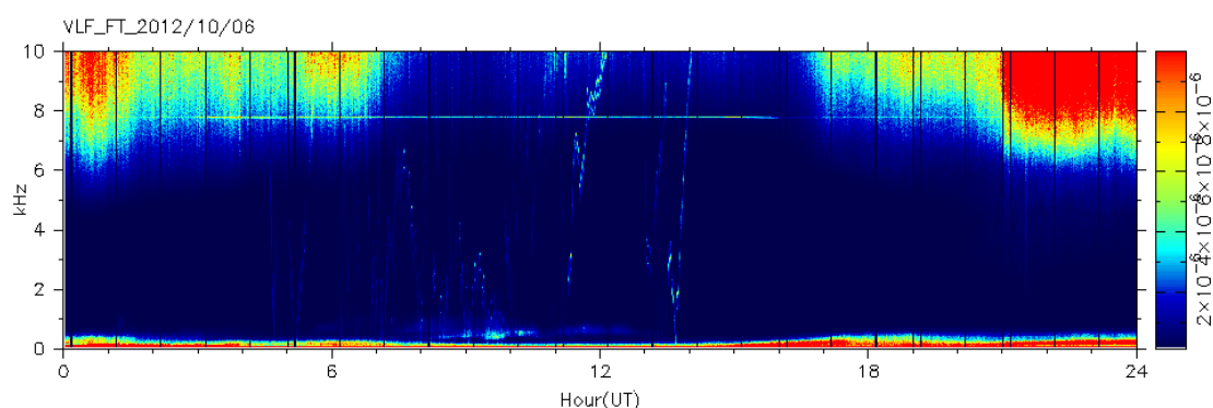
Figure 1. VLF Wide-band Spectrogram obtained by the new data logger deployed in West-ongul island. This spectrum is obtained in October 6, 2012.
