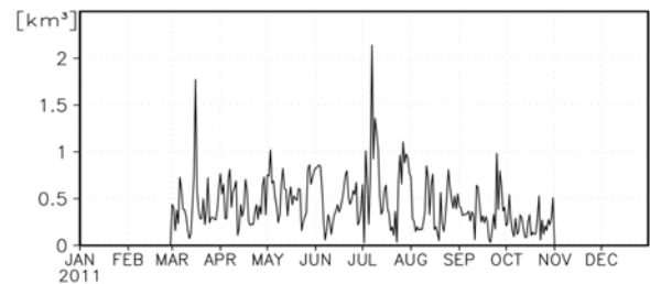
Fig. 3. Time variation of sea ice production in Vincennes Bay Polynya.
