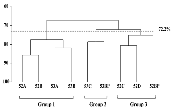
Figure 1. Dendrogram of the cluster analysis based on the Bray-Curtis similarity index with UPGMA linkage.
