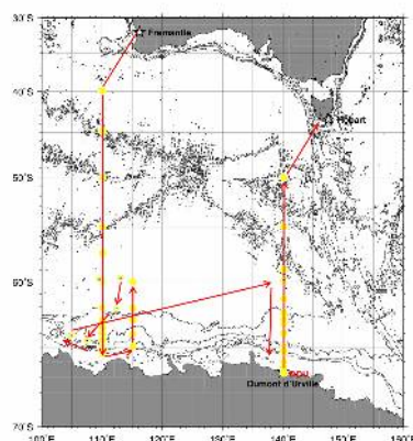
Fig. 1. Cruise track of JARE53 in the study sea area of the Southern Ocean.
