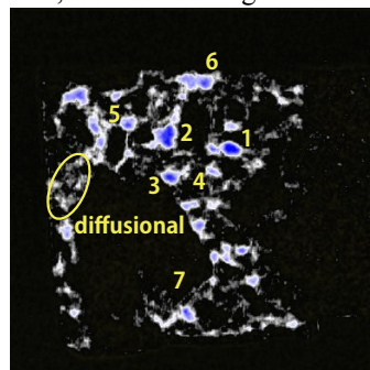
Fig. 2: Carbon elemental map of the specimen. Particulate and diffusional OM is indicated blue and white respectively.
