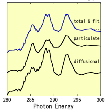
Fig. 3: C-XANES of diffusional OM, C-rich particulate, and total carbon region of thin section, from bottom to upper. Fitting line indicated as dotted line.
