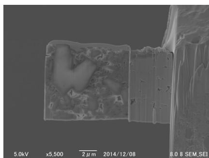
Fig. 1: SEM secondary electron image of the thin foil specimen for compact STXM.
