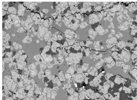
Fig. 2. Ca distribution map of Y002712. Abundant bright phases are augite. Medium-grey is maskelynite. Dark grey is pigeonite. The width of the image is 1.5 mm.
