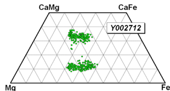
Fig. 3. Pyroxene quadrilateral of Y002712.
