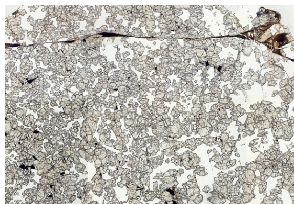
Fig. 1. Optical photomicrograph of Y002712 (plane-polarized light), showing the presence of abundant small pyroxene with interstitial maskelynite. The width of the image is ca. 4.5 mm.
