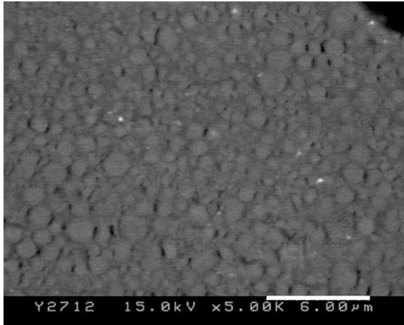
Fig. 4. Back-scattered electron image of a shock melt vein in Y002712, showing the presence of 1-2 \mu\text{m} aggregates of majorite. Scale bar is 6 \mu\text{m} .
