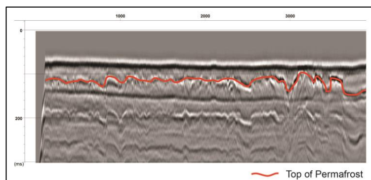
Figure 2. Stacked section showing the top of permafrost
