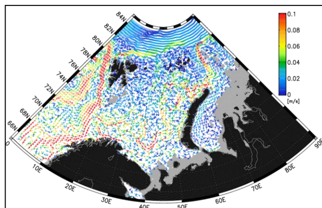
Figure 1: The simulated horizontal velocity (vector) at 50 m depth. The color of vector indicates the magnitude of horizontal velocity (m/s). The routes of Atlantic Water are captured by the bottom topography in Barents Sea.
