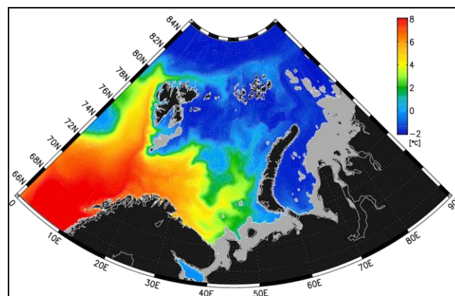
Figure 2: The simulated potential temperature at 50 m depth ( ^{\circ}\text{C} ). The warm Atlantic Water enters through the Barents Sea Opening and is cooled along its route in the Barents Sea.
