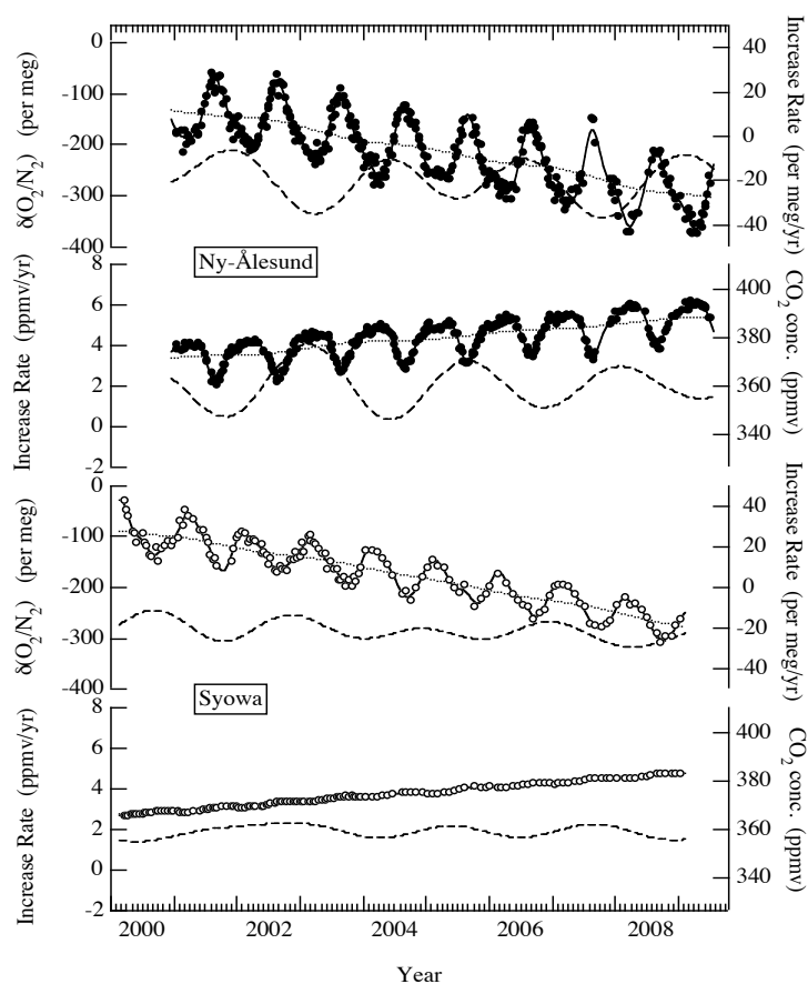
Figure 1. Variations of atmospheric δ(O 2 /N 2 ) and CO 2 concentration observed at Ny-Ålesund, Svalbard and Syowa Station, Antarctica. Closed and open circles are observed data and thick lines are best fit curves of the observed data. Thin lines and dashed lines represent secular trends and annual increase or decrease of the trends.
