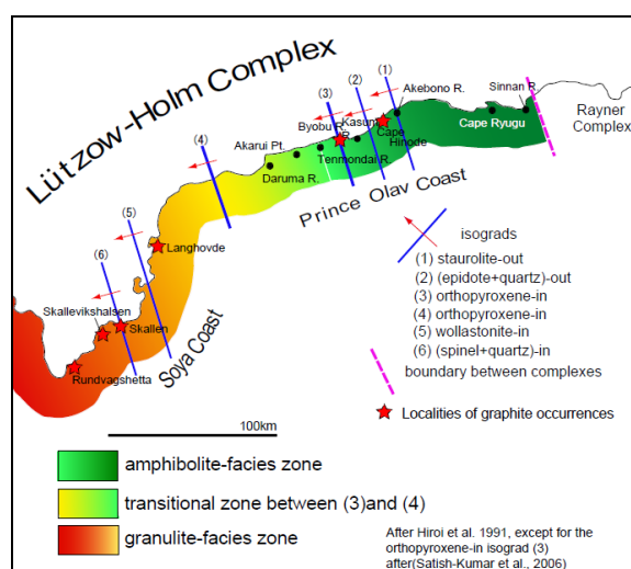
Figure 1. Simplified geological map of the Lützow-Holm Bay region. Progressive increase in metamorphic grade along the Prince Olav Coast to the Soya Coast is based on Shiraishi et al. (1989). Bold line show the isograds identified by Hiroi et al. (1991)
