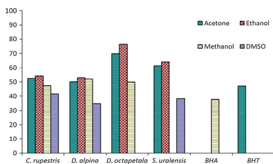
Fig1 Free radical scavenging activity of plant species in solvents. C. rupestris = Carex rupestris , D. alpina = Deschampsia alpina , D. octopetala = Dryas octopetala , S. uralensis = Silene uralensis . BHA = butylated hydroxyanisole, BHT = butylated hydroxytoluene, DMSO = dimethylsulfoxide
