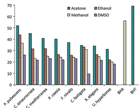
Fig.2 Free radical scavenging activity of lichen species in various solvents
