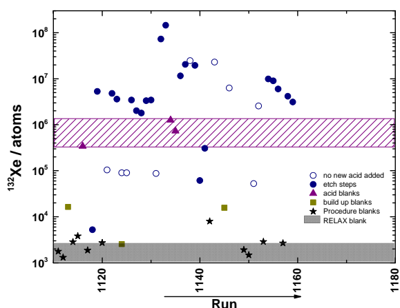
Fig. 2 Xe released during the etch run of 60 \mu\text{g} of aerogel compared to the RELAX, procedure, build-up and acid blanks.
