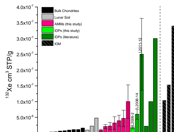
Fig. 1 Xe concentrations in IDPs and AMMs from this study compared with chondrites, lunar soil, IDPs from previous studies and IOM residues.
