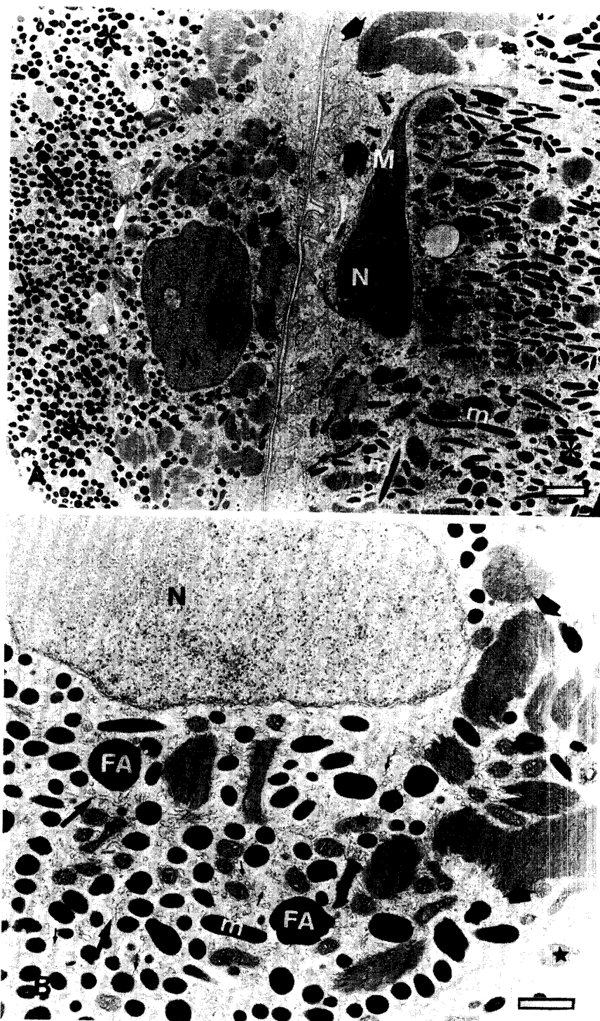
Fig. 2. Retina pigment epithelium in N. neglecta . A. general aspect of the pigment epithelium. Notice the infoldings of the plasma membrane (★), melanin pigment (*), melanosomes (m), and detached membranes of the external segment of photoreceptors (▲), the nucleus (N) and nucleolus (Nu) of the epithelial cells (scale: 2000 nm); B. Basal region of the pigment epithelium with phagosomes (FA), melanosomes (m), detached membranes of photoreceptors (▲), nucleus (N), mitochondria (★), smooth endoplasmic reticulum (▼) and microtubules (↓) all over the cytoplasm. (scale 1000 nm).
