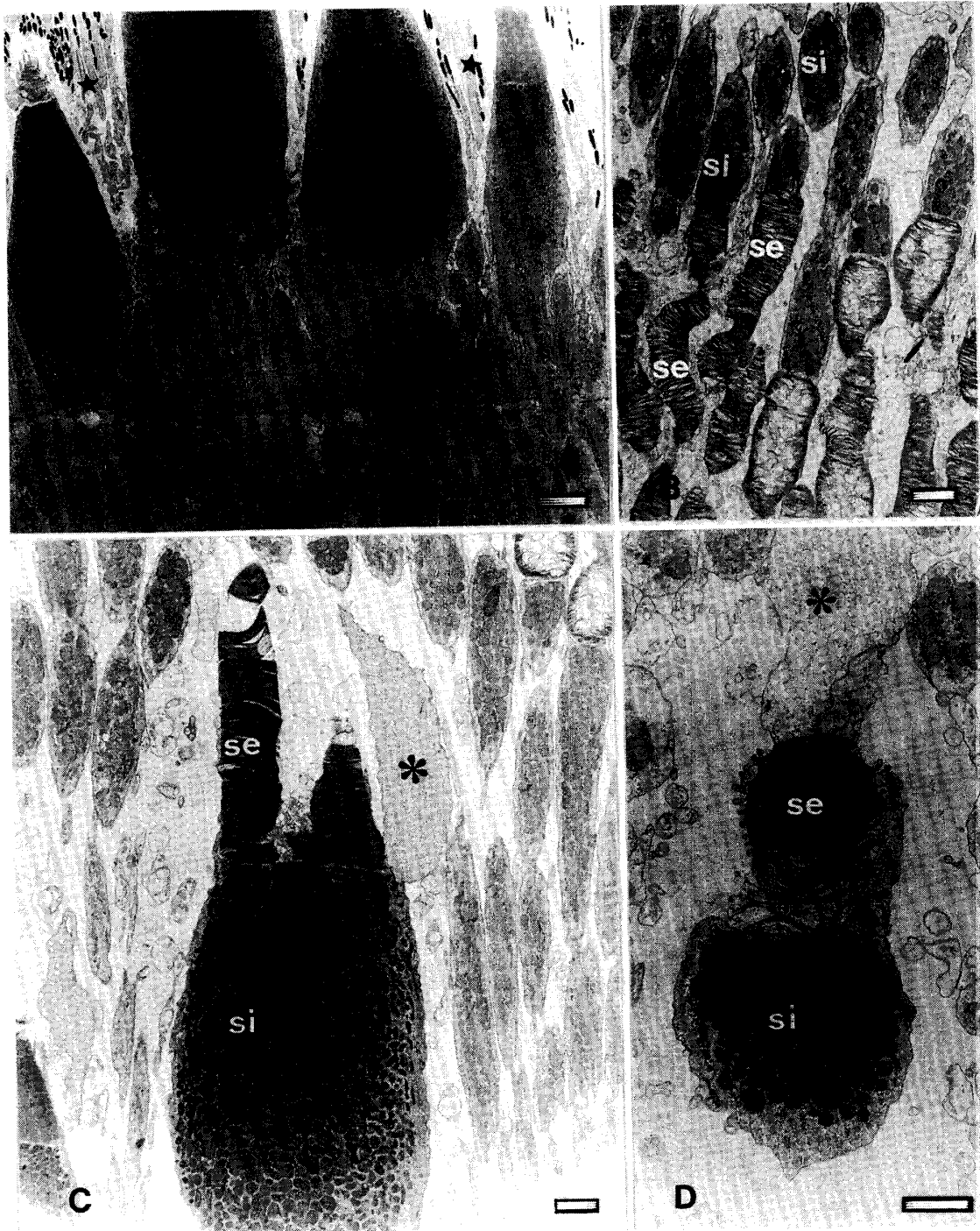
Fig. 3. Detail of the retina in N. neglecta . A. general view of some photoreceptors with outer nuclear layer (↑), outer limiting membrane (↑), cones (✱) and rods (★) (scale: 7000 nm); B. Rods with inner segment (si) and outer segment (se) (scale: 2000 nm); C. Double cones with inner segment (si), outer segment (se), and accessory outer segment (✱) (scale: 2000 nm); D. Single cones with inner segment (si), outer segment (se), and accessory outer segment (✱) (scale: 2000 nm).
