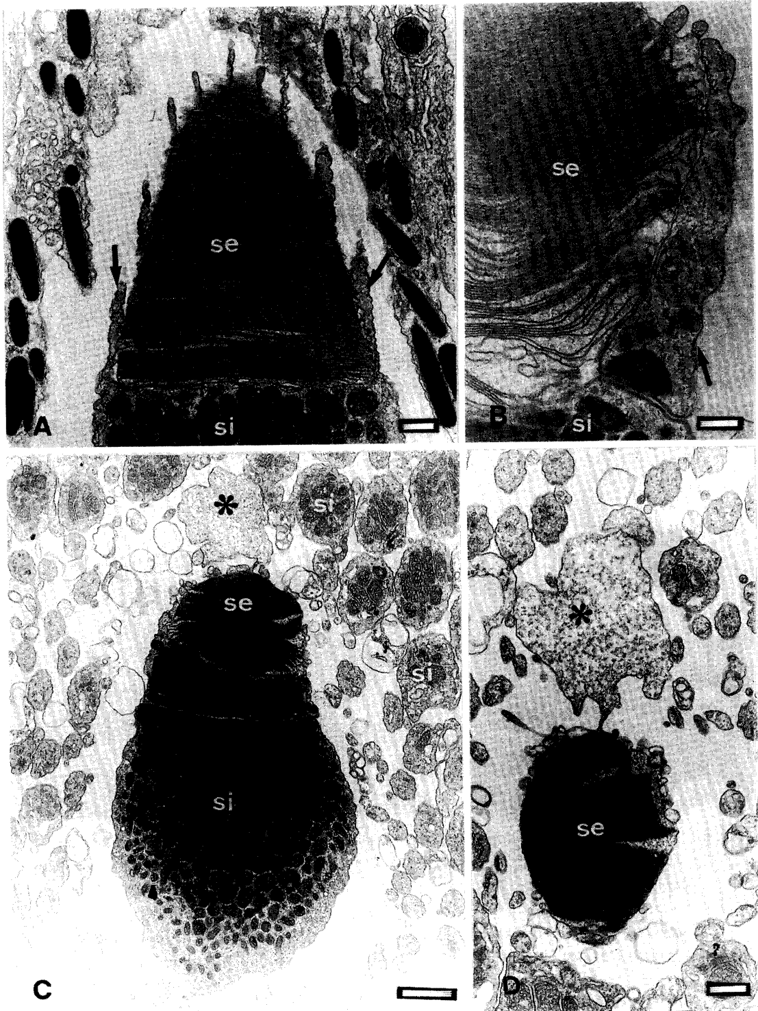
Fig. 7. Calycal processes and accessory outer segments in cones of Notothenia neglecta . A. Calycal processes ( \downarrow ) surrounding the outer segment (se) of a cone. Notice the inner segment (si) rich in mitochondria ( \star ) and the outer segment with bimembranous lamellae ( \star ) (scale: 500 nm); B. detail of the calycal process ( \uparrow ), inner segment (si) and outer segment (se) (scale: 500 nm); C. outer accessory segment ( \star ), outer segment (se) and inner segment (si) (scale: 2000 nm); D. outer accessory segment ( \star ) and its connection with the outer segment of the cone (se) (scale 1000 nm).
