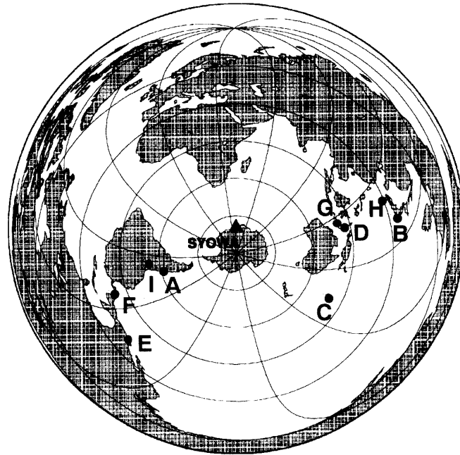
Fig. 5. Epicentral distributions of earthquakes recorded at Padda Island and Strandnebbba.
