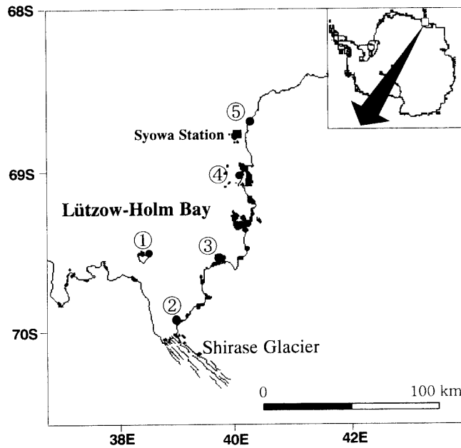
Fig. 1. Location of the observation points. Numbers indicate the following observation points: 1) Padda Island, 2) Strandnebba, 3) Skallen, 4) Langhovde, 5) Tottuki Point. Details of each station are referred to Table 1.
