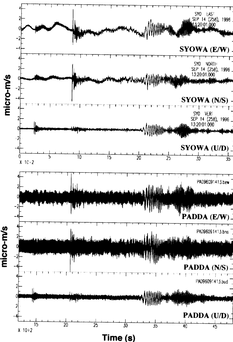
Fig. 6. Observed waveforms of the earthquake which occurred in the Santa Cruz Island region recorded at Syowa Station (upper plot) and at Padda Island (lower plot).
