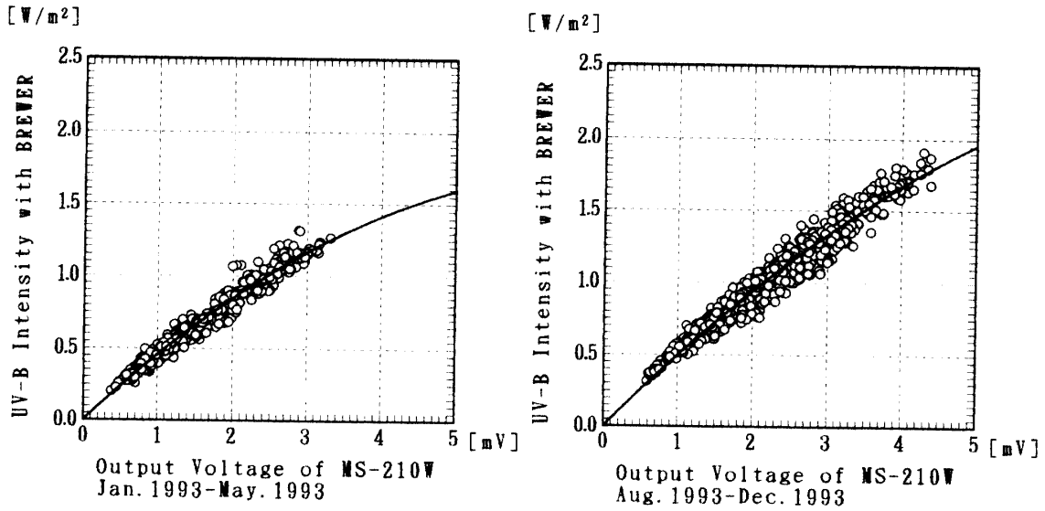
図 19 紫外域日射計の出力電圧と Brewer 分光光度計による UV-B 強度との関係 Fig. 19. The relation between output voltage with global UV-B radiometer and UV-B intensity with Brewer spectrophotometer. The solid line shows a quadratic approximation by the method of least squares.
