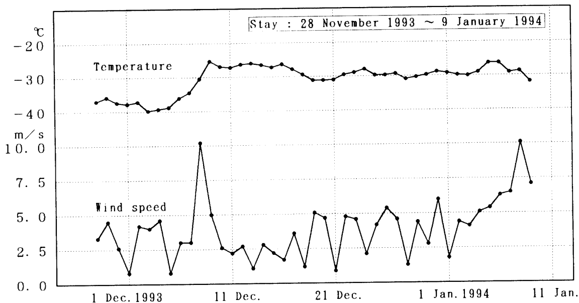
図 30 ドームふじ観測拠点滞在中の気温と風速 (15LT) Fig. 30. Temperature and wind speed during stay at Dome Fuji Station.
