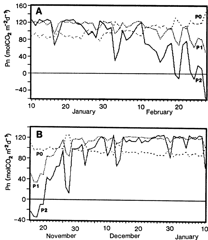
Fig. 6. Diel net photosynthetic rates ( P_n ) of P0, P1 and P2 samples in the periods from 10 January to 27 February 1988 (A) and from 16 November 1988 to 10 January 1989 (B).
