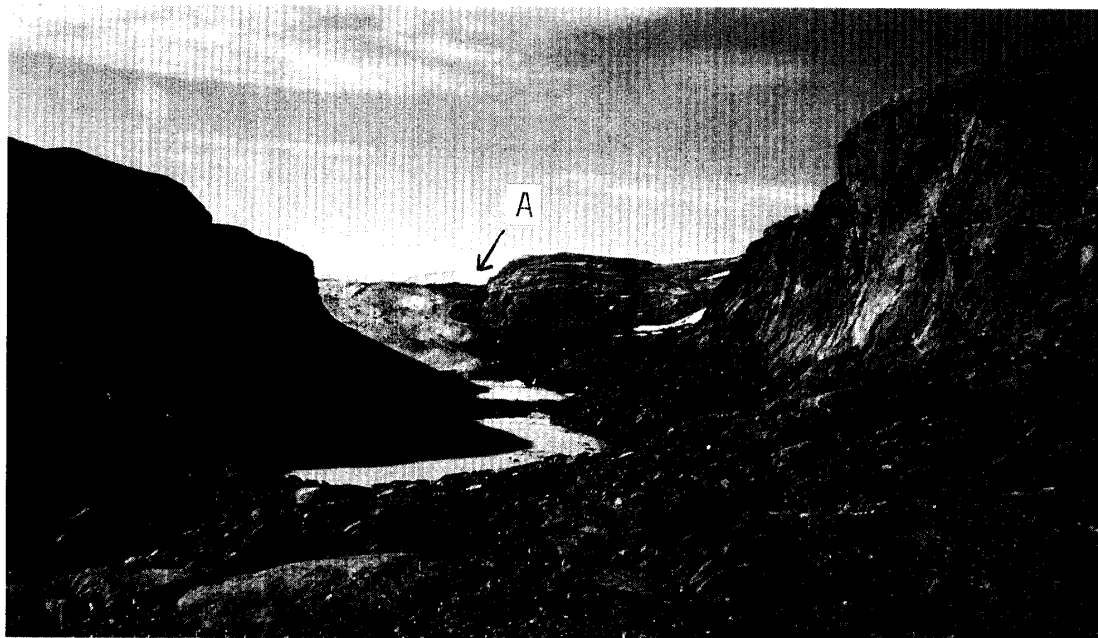
Fig. 5. A hollow with nearly vertical sidewalls and frozen lakes. Scattered erratics exist on the bottom. Looking northward. A: shear moraine currently being formed.
