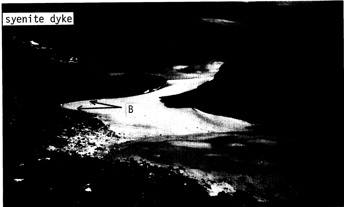
Fig. 6. Two protilus ramparts (indicated by B) in a hollow at the eastern part of the northern Balchenfjella. An ice tongue from the Oberstbreen still spills into this hollow. A syenite dyke indicated.
