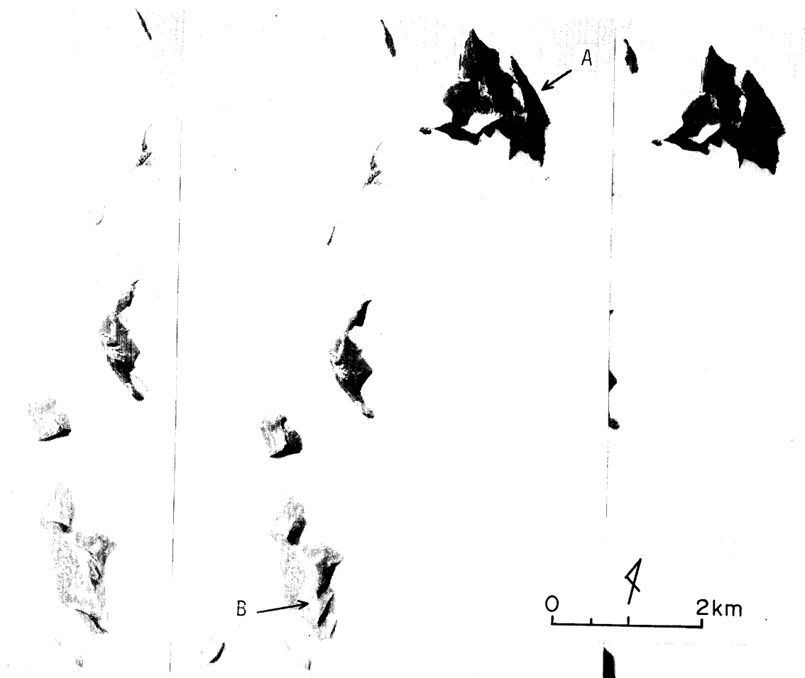
Fig. 11. Stereogram of Austhjelm (a northern nunatak) and Hettene (southern nunataks). Note: very extensive development of wind scoops, particularly on the east. A: rectilinear slope at Austhjelm. B: probable rock glacier at Hettene.
