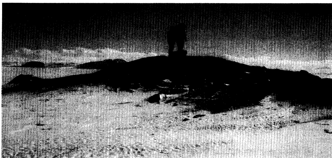
Fig. 9. A tiny outcrop of the ice-free area at the southern end of the southern Balchenfjella. Persons for scale. The outcrop seems to have been caused by very recent deglaciation; however, bedrocks and rock fragments on them are very much weathered. The ice-free area in the back is Gunnar Isachsenfjellet.
