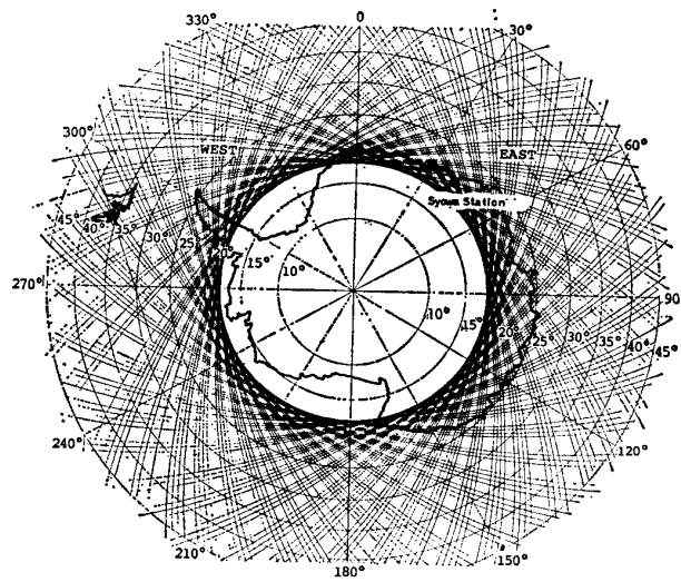
Fig. 5. Orbits of SEASAT around Antarctica south of 45° S.
