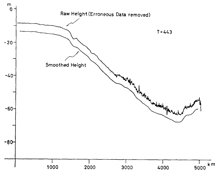
Fig. 4. A profile of raw altimetry data (upper) showing the effect of ice pack in the winter Antarctic sea. The lower profile is a result of smoothing, which is 5 m apart from the profile of the raw data for readability.
