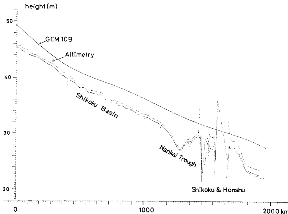
Fig. 1. An example of the SEASAT altimetry data along the orbits across the Shikoku Basin. Left—south, right—north.
