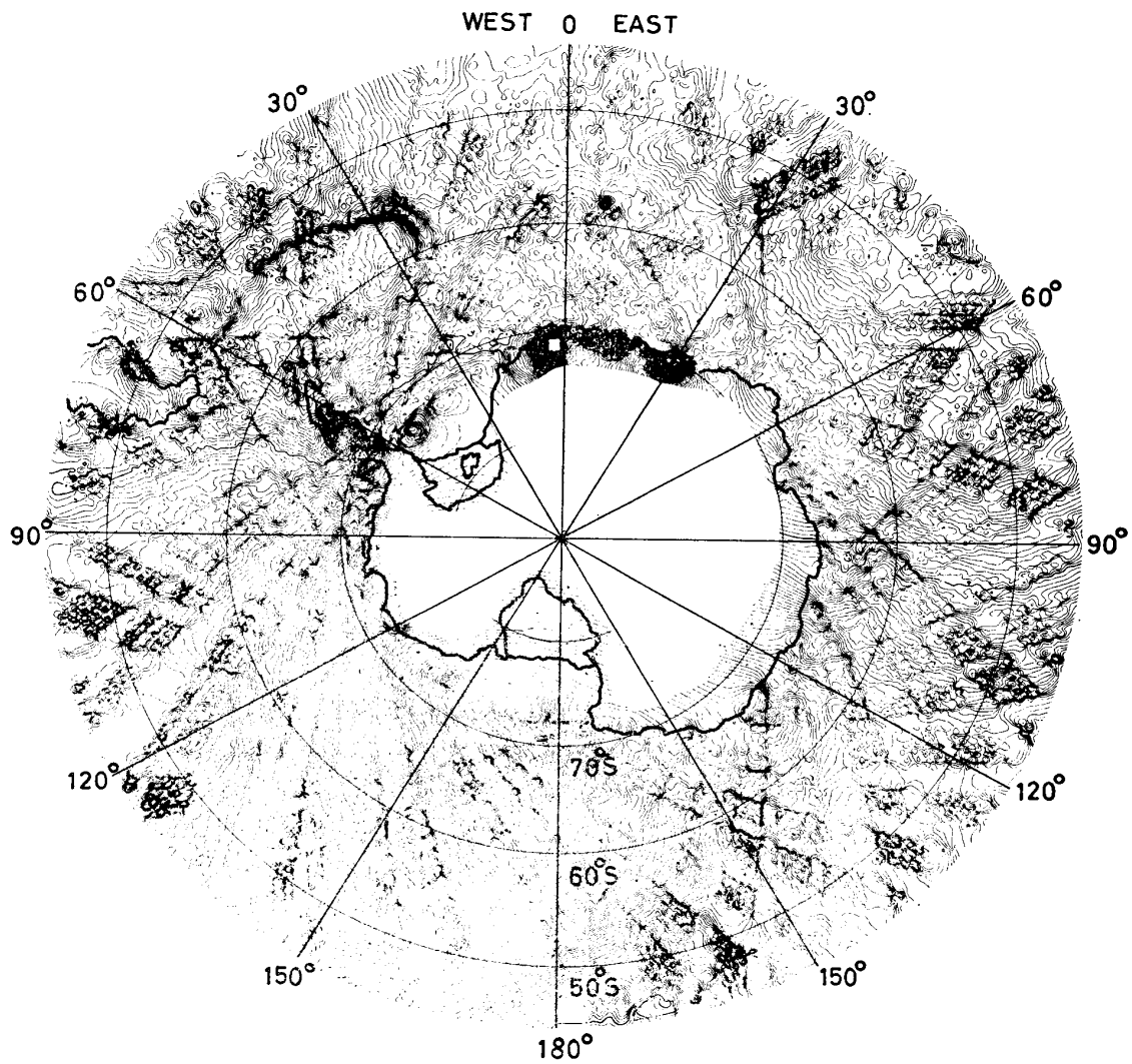
Fig. 6. Contours of sea surface topography with an interval of 1 meter around the Antarctic Continent. Satellite orbits are seen obviously.
