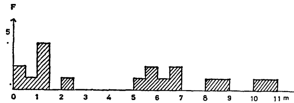
Fig. 2. Distribution of height differences of the SEASAT altimetry at orbital crossings.
