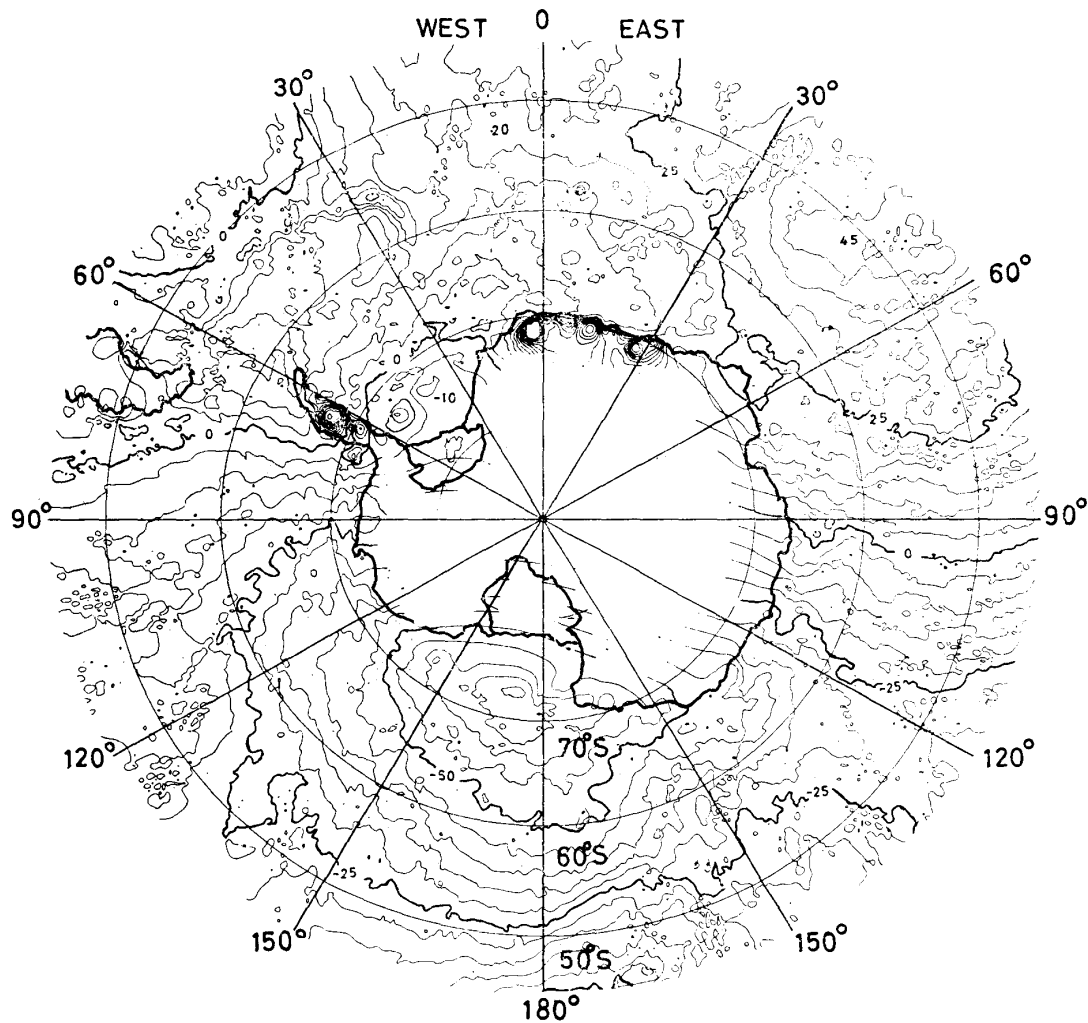
Fig. 7. Contours of sea surface topography with an interval of 5 m.
