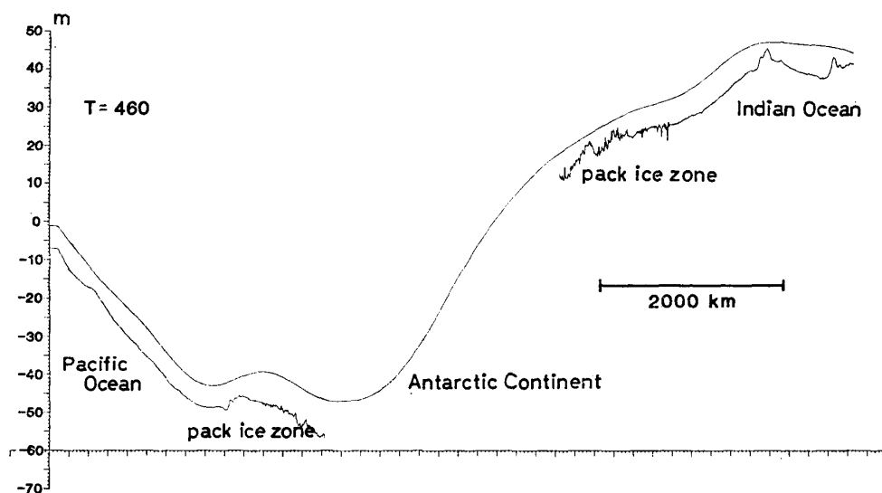
Fig. 3. A profile of the SEASAT altimetry (lower) vs. a corresponding profile of GEM 10B geoid across the Antarctic Continent in the winter season. The profile is along orbit No. 460.
