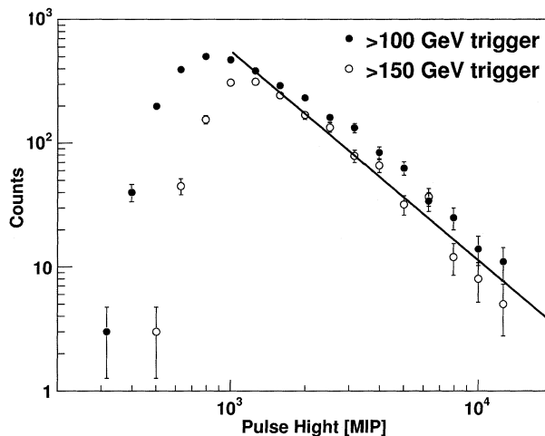
Fig. 10. Pulse height distributions observed by the scintillation counter placed at depth of 7 r.l. for the 100 GeV threshold (black dots) and for the 150 GeV threshold (open circles). The solid line shows a power law spectrum with an index of -2.7 .
