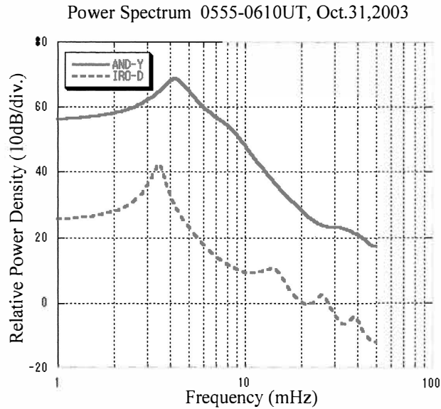
Fig. 8. Comparison of power spectra of the Y and D component magnetic field Pc 5 oscillations during the interval of 15 min from 0555 UT to 0610 UT indicated with the dotted vertical lines in the previous figure, observed at Andenes (solid curve) and Iriomote (dotted curve). Spectral peaks stand at about 4 mHz. However, the power is larger with approximately 20 dB at Andenes compared with that at Iriomote.
