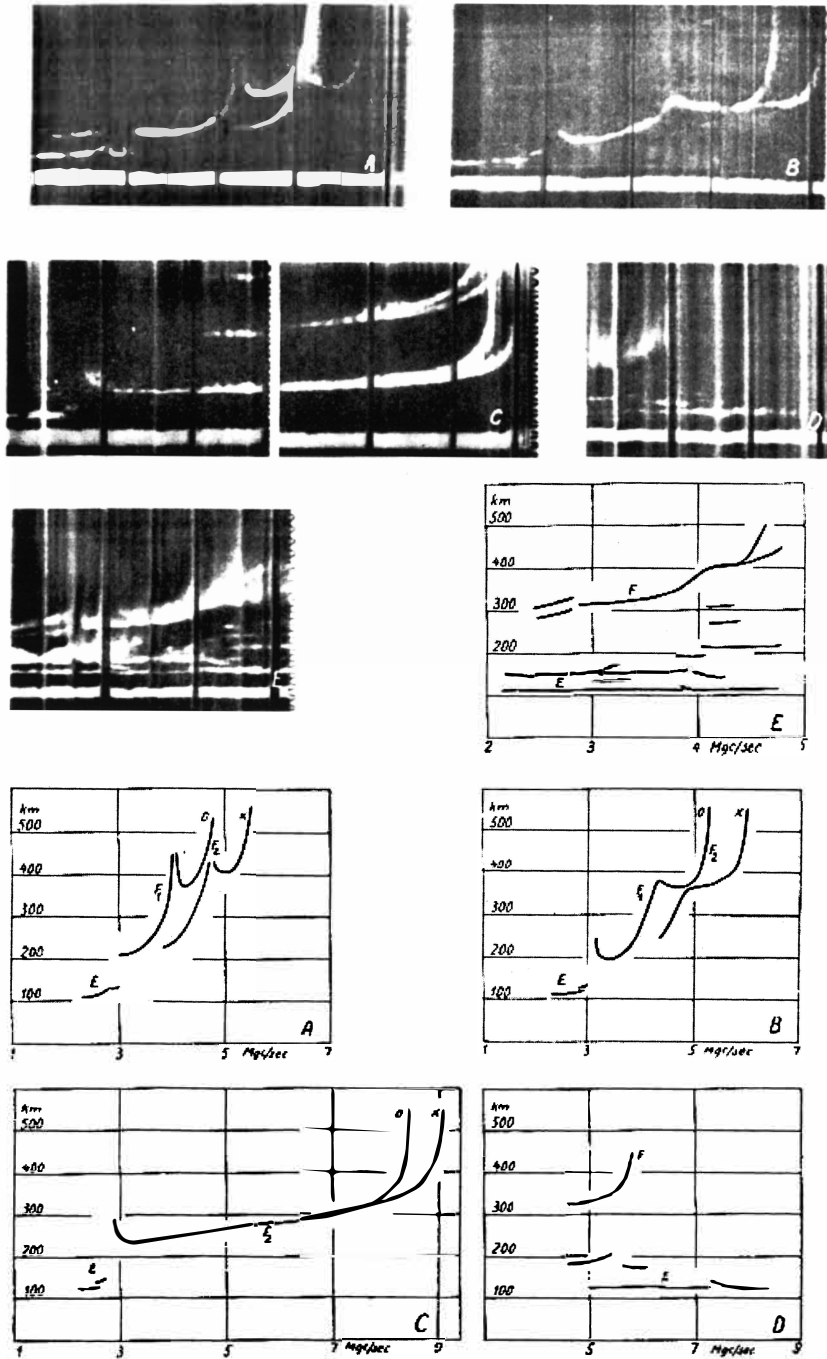
Fig. 3. Early results from the first Norwegian ionosonde on a variety of days between May 1935 and October 1936. The line drawings show the operators' interpretations of the echoes, and, importantly, the calibrations necessary for any re-analysis of the archived photographic recordings (Harang, 1937).
